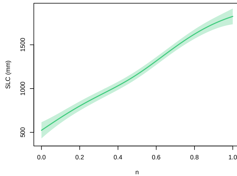
tas+thetao – parameter main effects at 2300 (other params at 0.5; forcing at EC-Earth3-Veg, ssp585)
