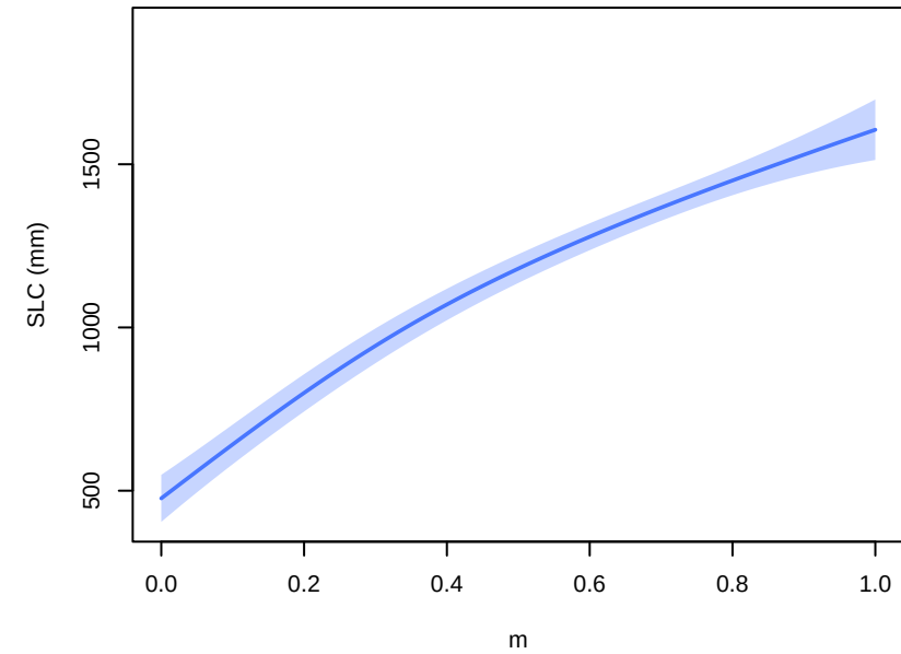
GMSTa+thermal_forcing – parameter main effects at 2300 (other params at 0.5; forcing at EC–Earth3–Veg, ssp585)
