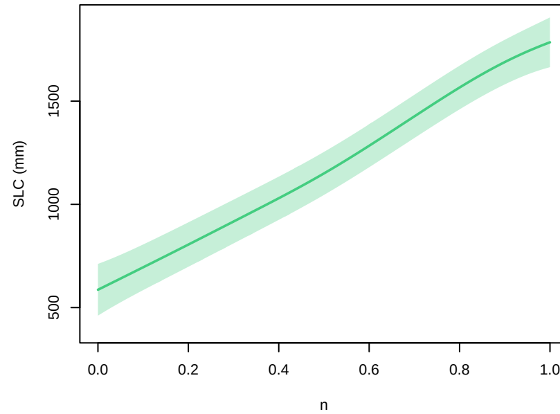
thermal_forcing – parameter main effects at 2300 (other params at 0.5; forcing at EC–Earth3–Veg, ssp585)
