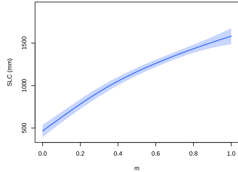
GMSTa+thetao – parameter main effects at 2300 (other params at 0.5; forcing at EC-Earth3-Veg, ssp585)
