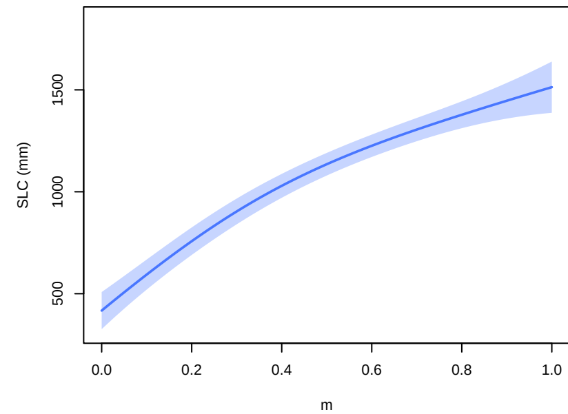
smb+thermal_forcing – parameter main effects at 2300 (other params at 0.5; forcing at EC–Earth3–Veg, ssp585)
