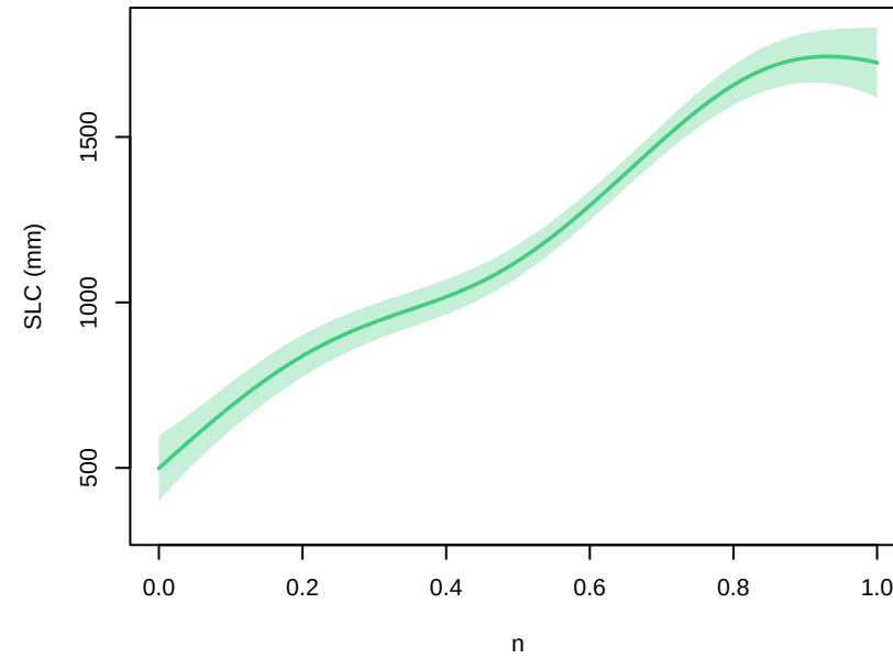
tas – parameter main effects at 2300 (other params at 0.5; forcing at EC–Earth3–Veg, ssp585)
