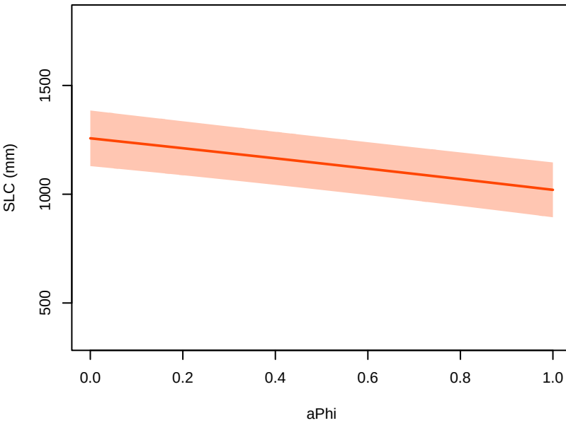
smb – parameter main effects at 2300 (other params at 0.5; forcing at EC–Earth3–Veg, ssp585)
