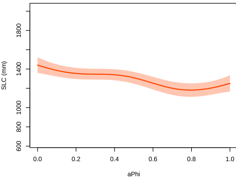
tas+thetao – parameter main effects at 2300 (other params at 0.5; forcing at MIROC-ES2L, ssp585)
