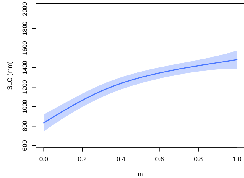
thetao – parameter main effects at 2300 (other params at 0.5; forcing at MIROC-ES2L, ssp585)
