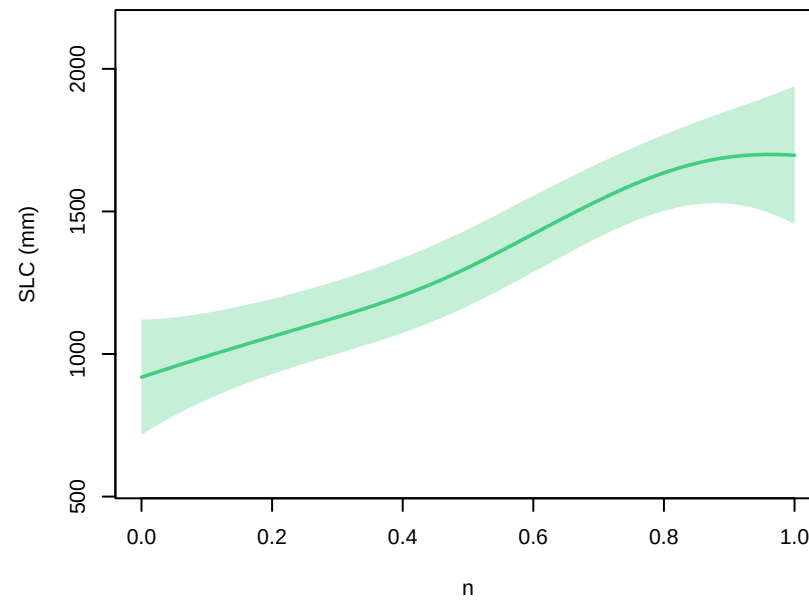
smb – parameter main effects at 2300 (other params at 0.5; forcing at MIROC-ES2L, ssp585)
