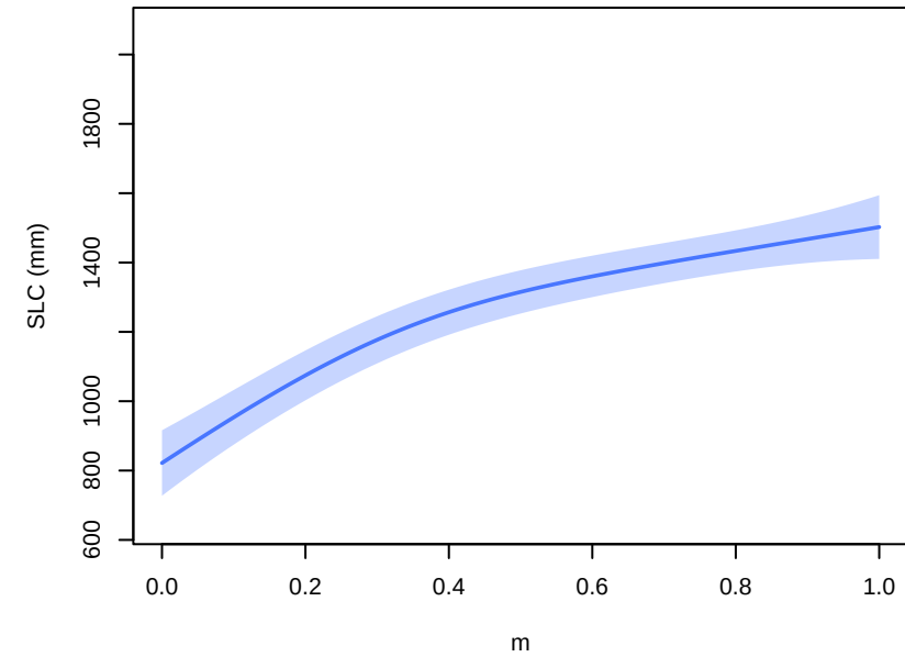
GMSTa+thetao – parameter main effects at 2300 (other params at 0.5; forcing at MIROC-ES2L, ssp585)
