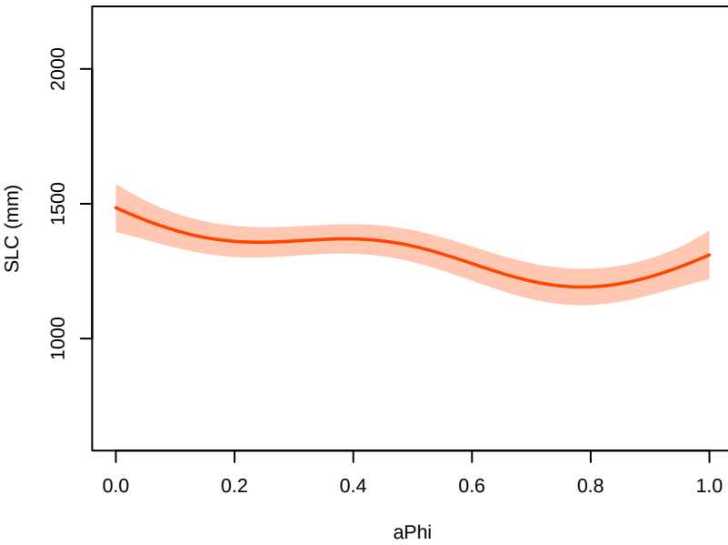
GMSTa+thermal_forcing – parameter main effects at 2300 (other params at 0.5; forcing at MIROC-ES2L, ssp585)
