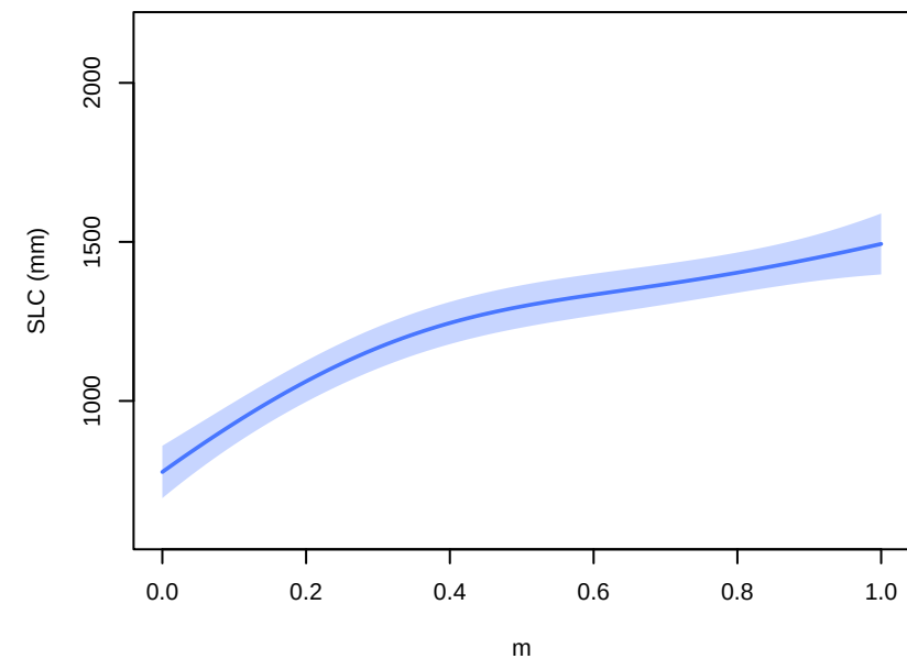
smb+thermal_forcing – parameter main effects at 2300 (other params at 0.5; forcing at MIROC-ES2L, ssp585)
