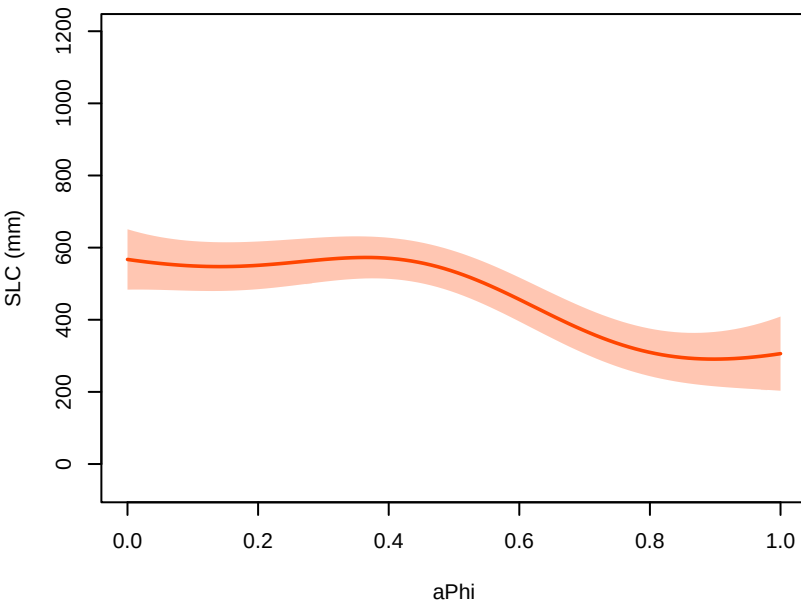
tas+thetao – parameter main effects at 2300 (other params at 0.5; forcing at MRI-ESM2-0, ssp585)
