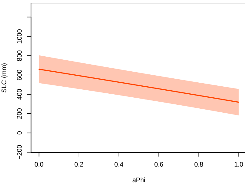
smb – parameter main effects at 2300 (other params at 0.5; forcing at MRI-ESM2-0, ssp585)
