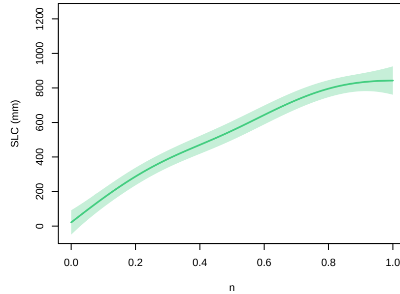
GMSTa+thetao – parameter main effects at 2300 (other params at 0.5; forcing at MRI-ESM2-0, ssp585)
