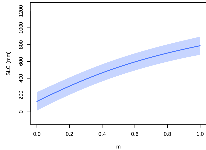
thermal_forcing – parameter main effects at 2300 (other params at 0.5; forcing at MRI–ESM2–0, ssp585)
