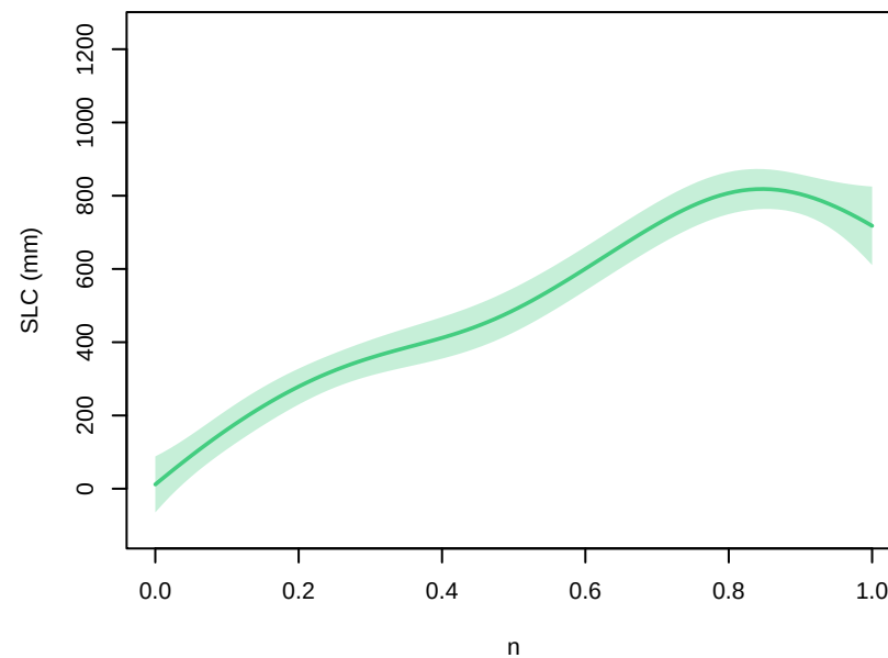
smb+thermal_forcing – parameter main effects at 2300 (other params at 0.5; forcing at MRI-ESM2-0, ssp585)
