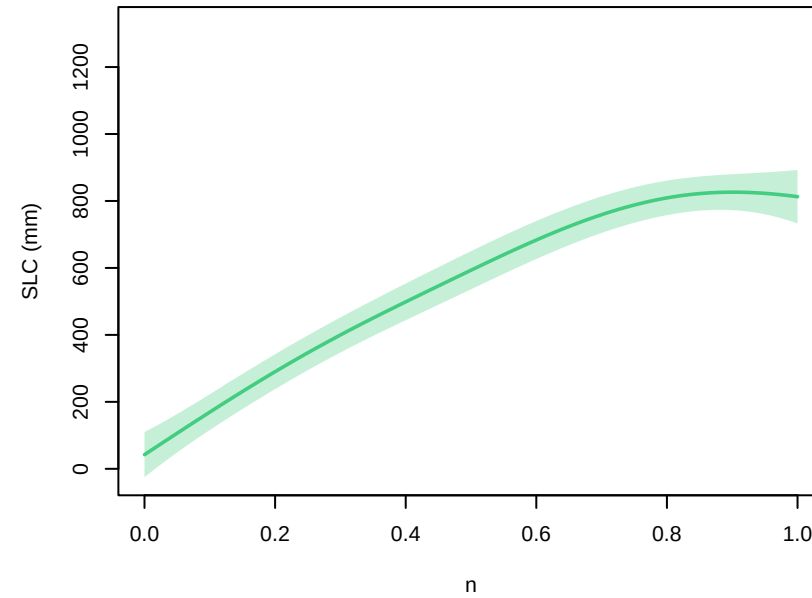
GMSTa+thermal_forcing – parameter main effects at 2300 (other params at 0.5; forcing at MRI-ESM2-0, ssp585)
