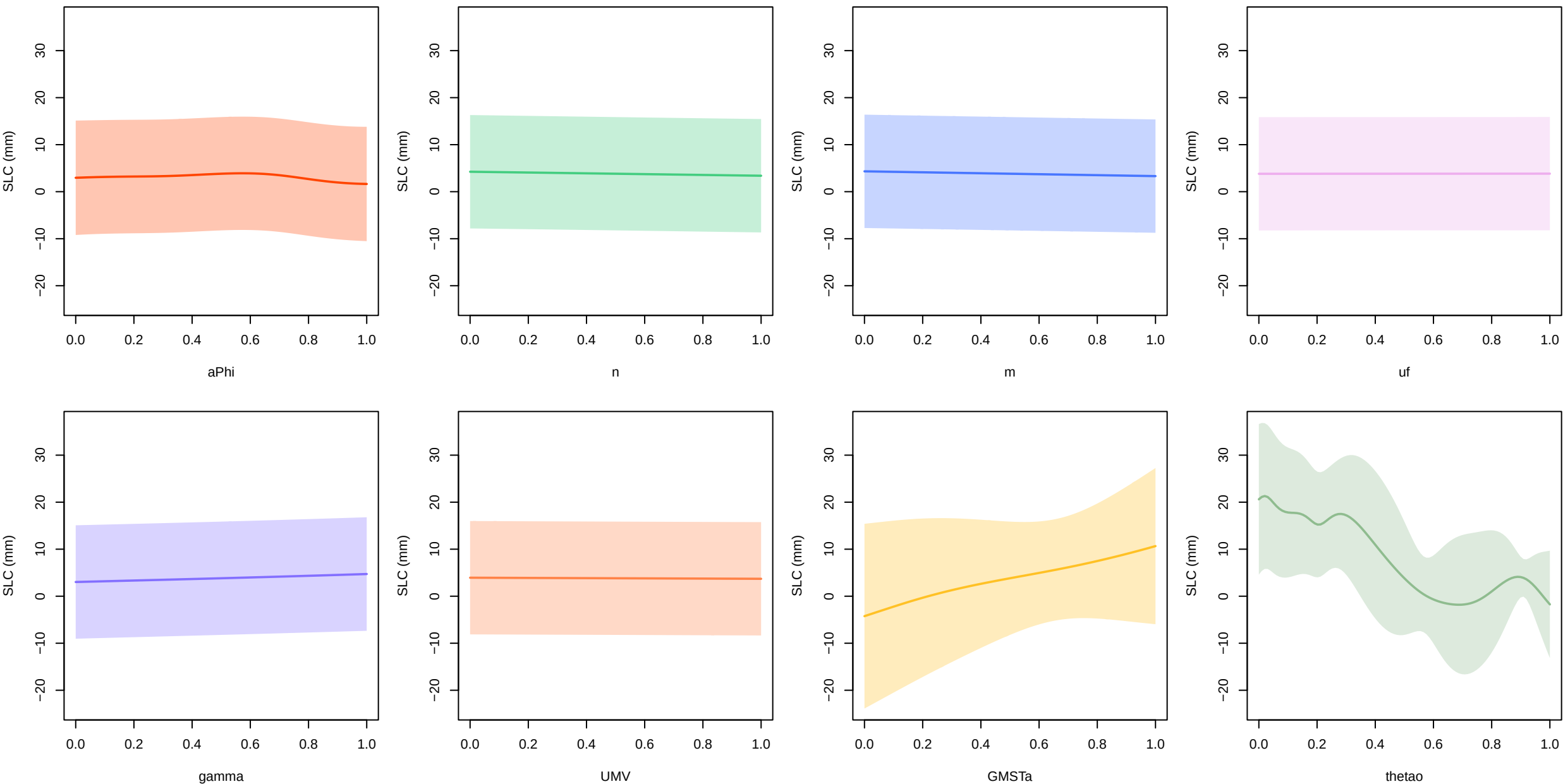
GMSTa+thetao – main effects at 2021 (all other inputs fixed at 0.5)
