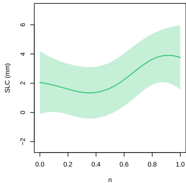
thermal_forcing – main effects at 2021 (all other inputs fixed at 0.5)
