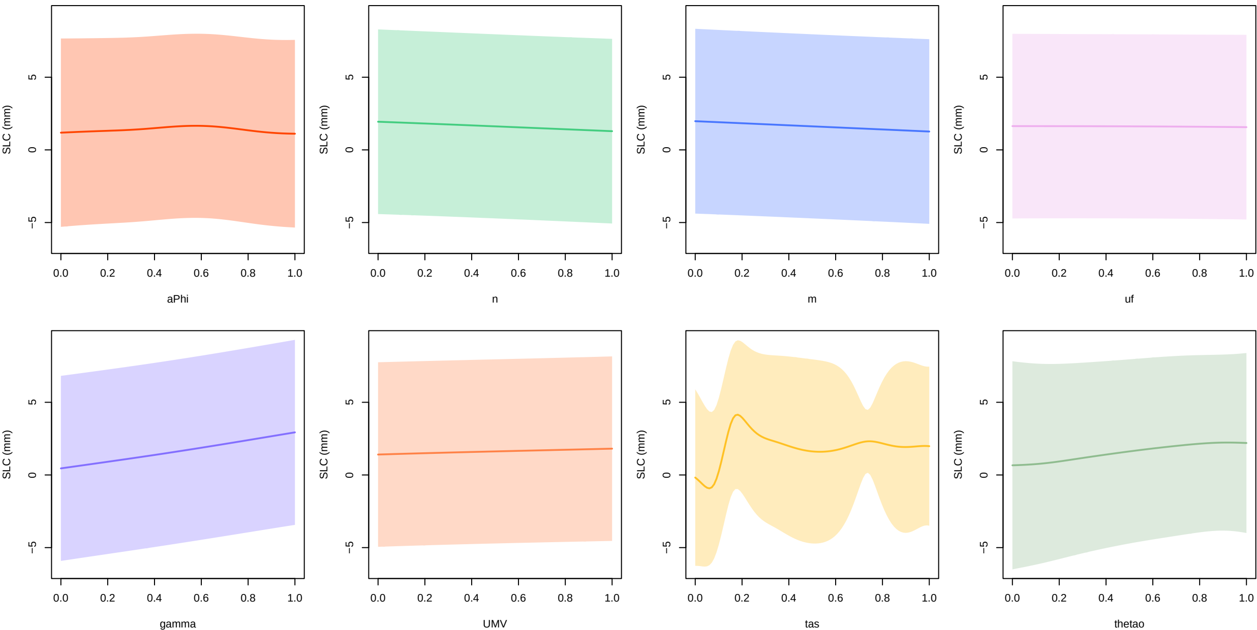
tas+thetao – main effects at 2021 (all other inputs fixed at 0.5)
