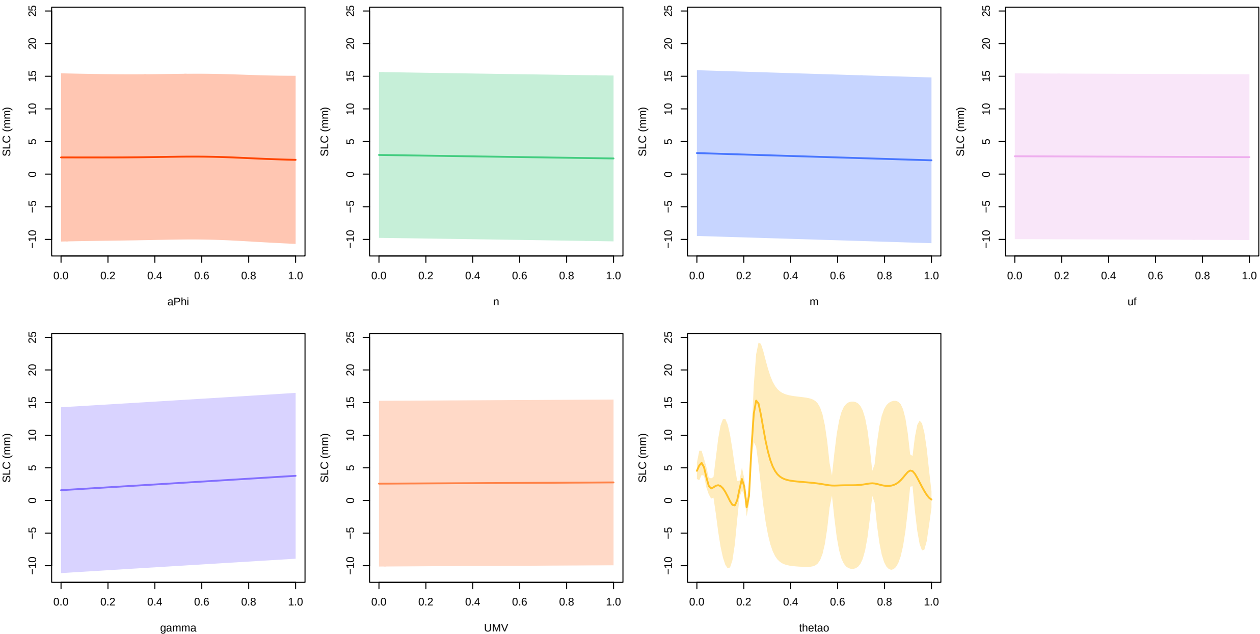
thetao – main effects at 2021 (all other inputs fixed at 0.5)
