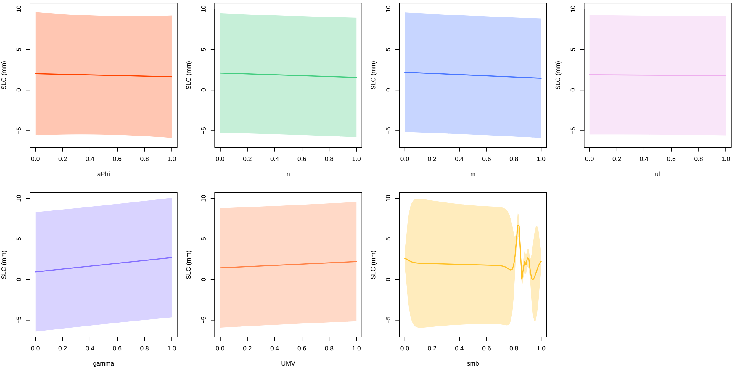
smb – main effects at 2021 (all other inputs fixed at 0.5)
