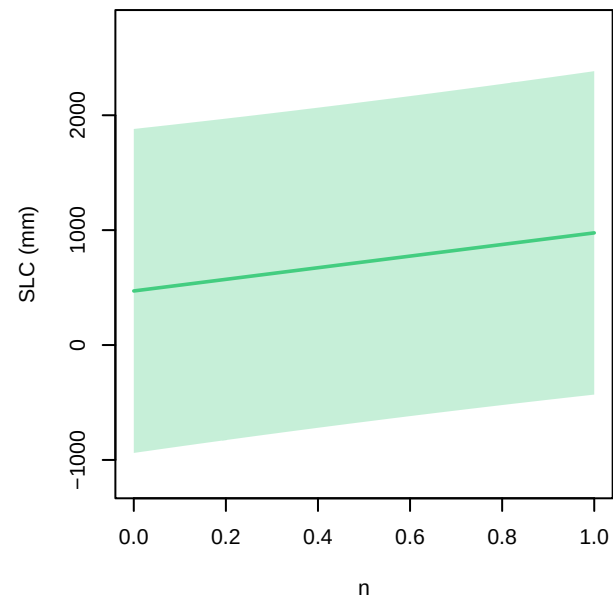
smb – main effects at 2300 (all other inputs fixed at 0.5)
