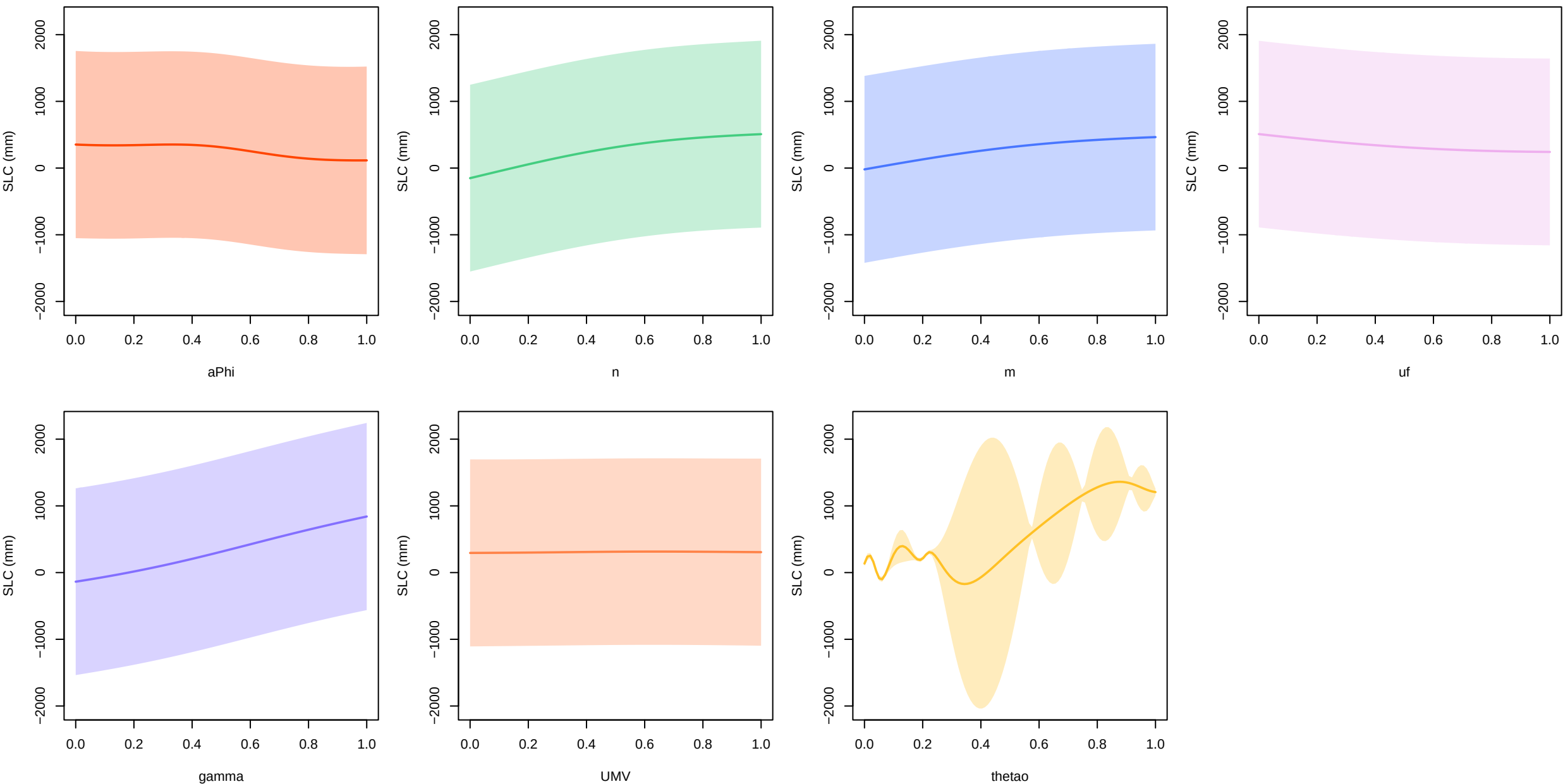
thetao – main effects at 2300 (all other inputs fixed at 0.5)
