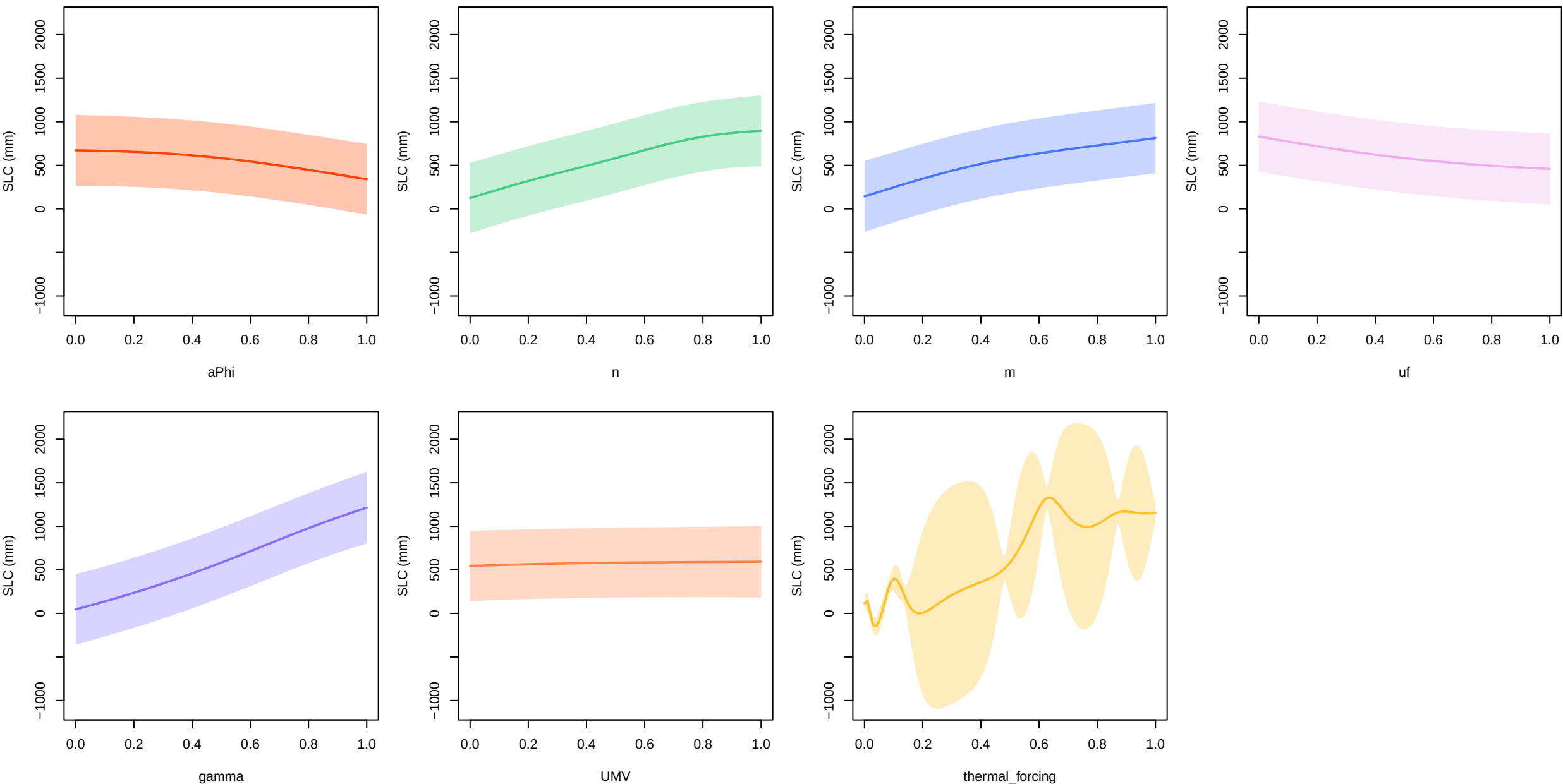
thermal_forcing – main effects at 2300 (all other inputs fixed at 0.5)
