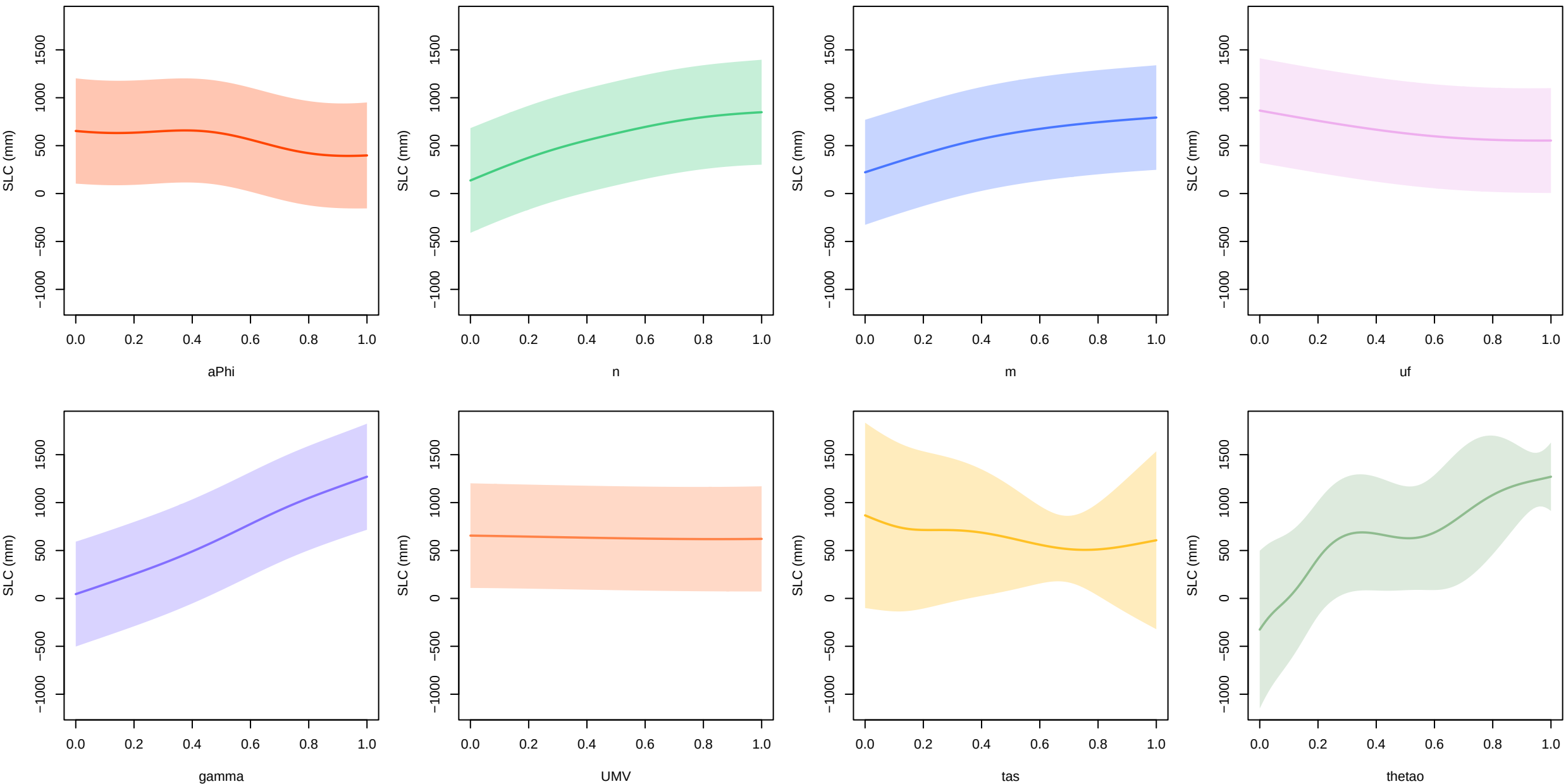
tas+thetao – main effects at 2300 (all other inputs fixed at 0.5)
