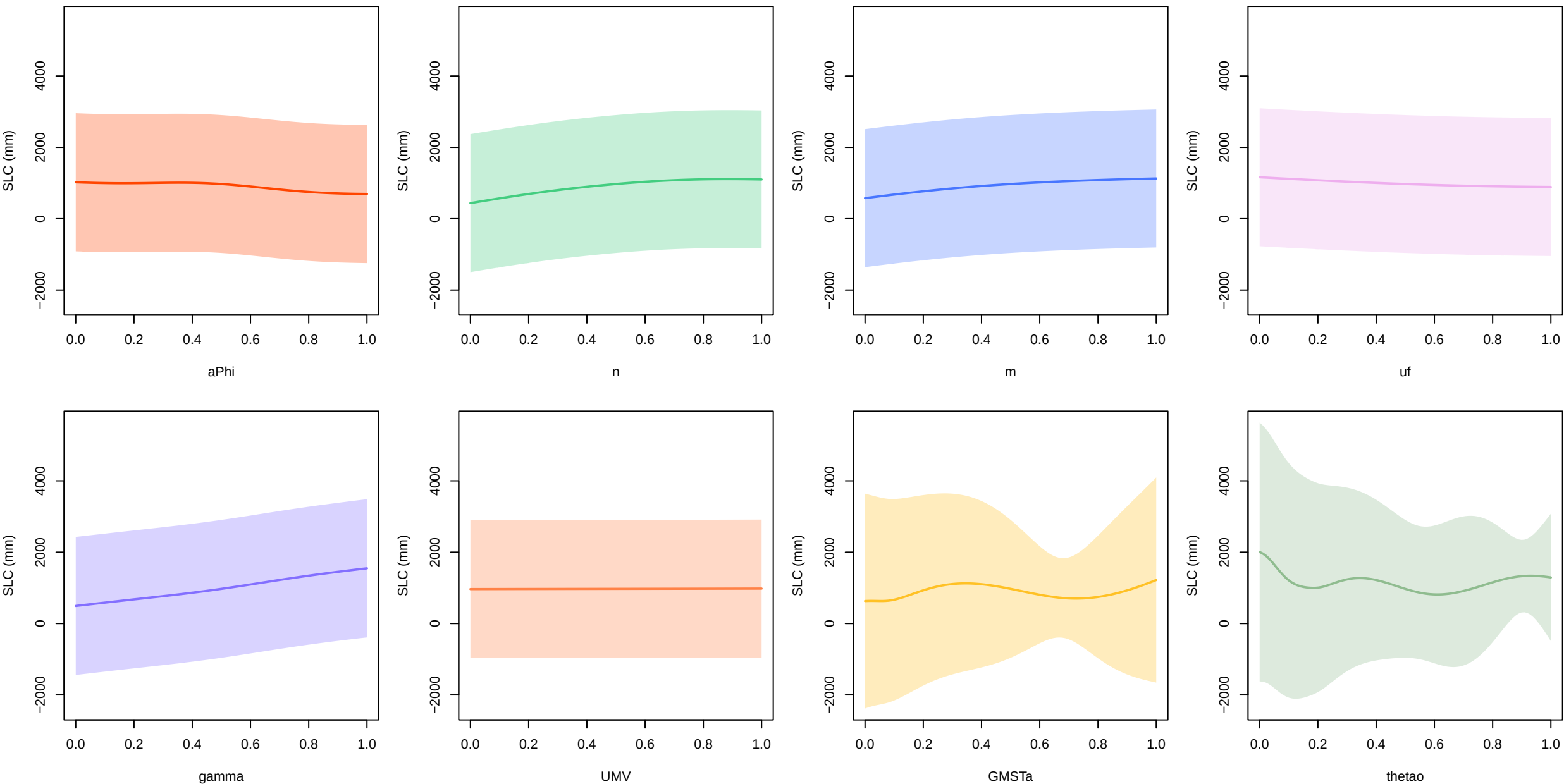
GMSTa+thetao – main effects at 2300 (all other inputs fixed at 0.5)
