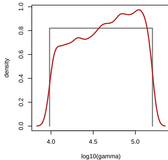
MRI-ESM2-0 - gamma
