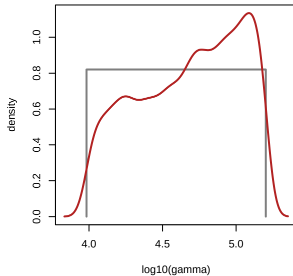
EC-Earth3-Veg - gamma
