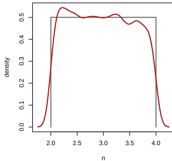
MRI-ESM2-0 - n
