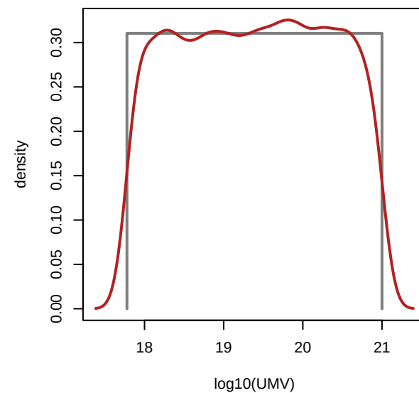
MRI-ESM2-0 - UMV
