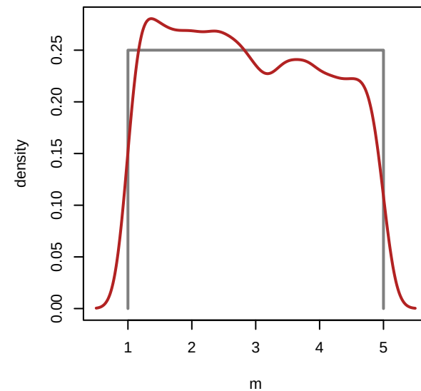
MRI-ESM2-0 - m
