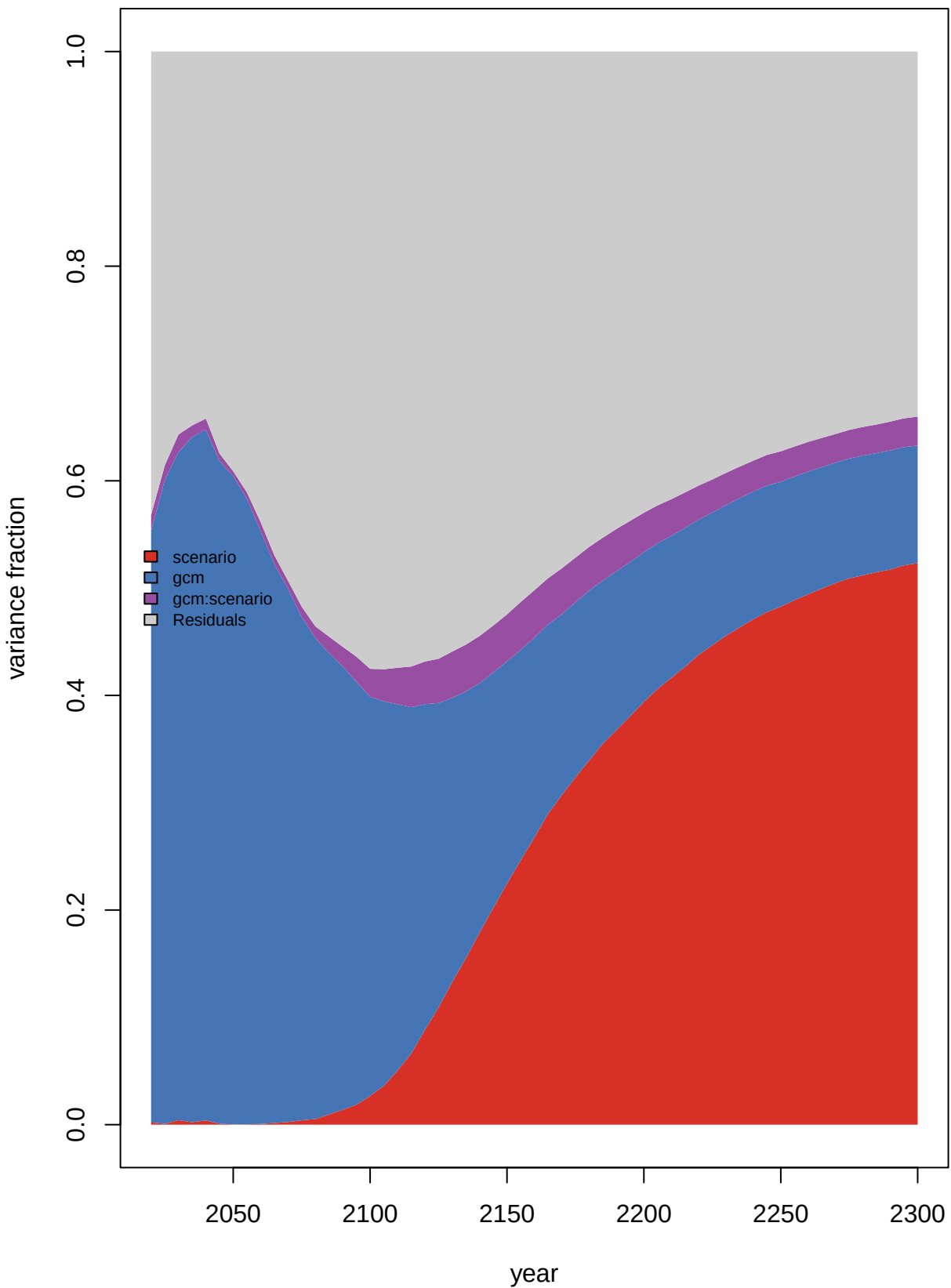
ANOVA: discrete factors (all scenarios)
