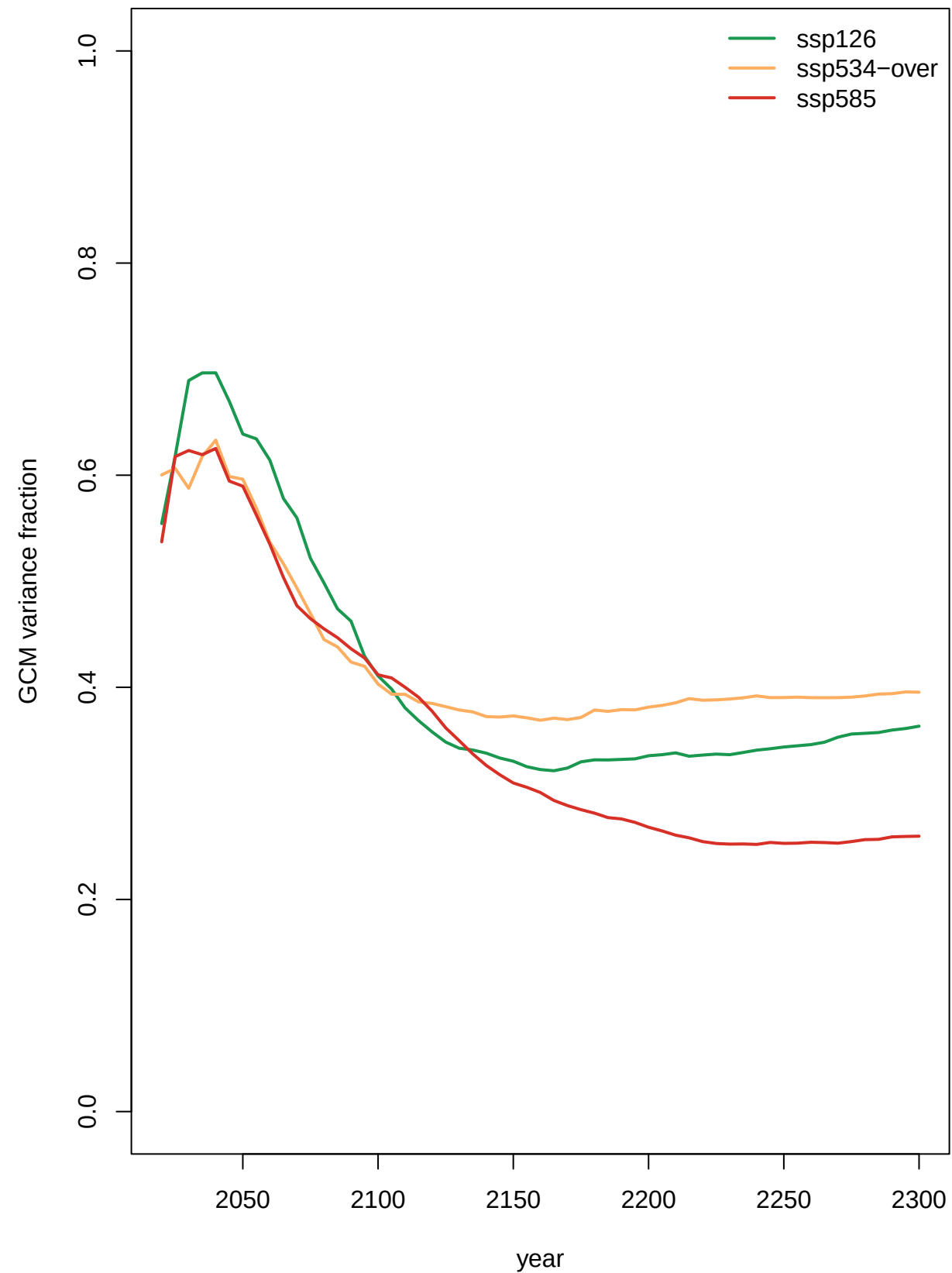
Per-scenario ANOVA: GCM share
