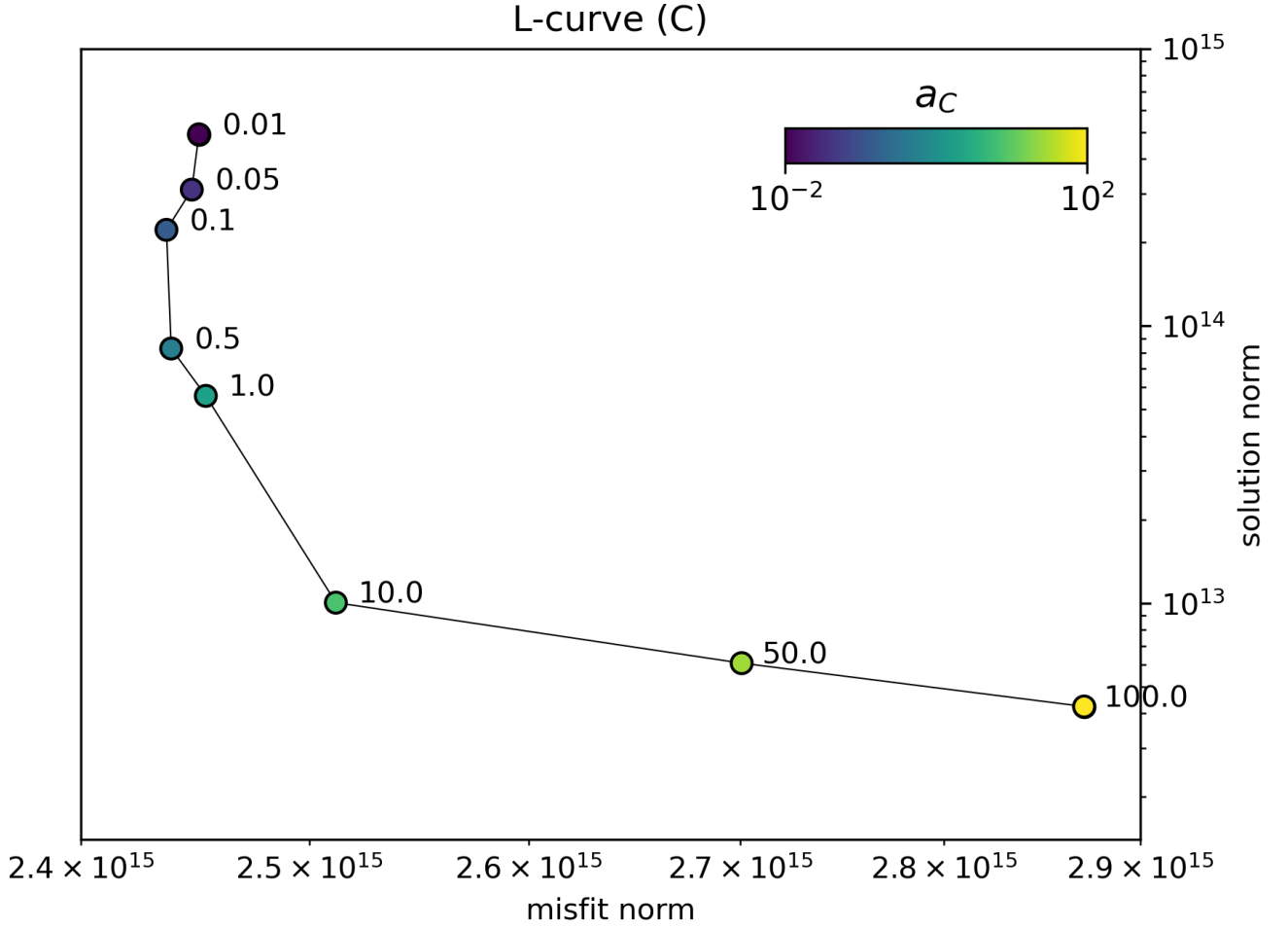
Figure 1. L-curves
