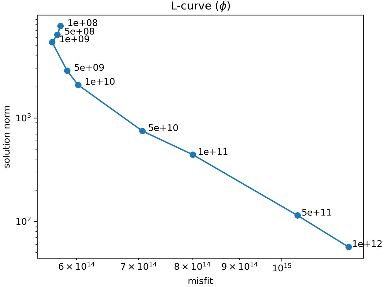
Figure 2. L-curves
