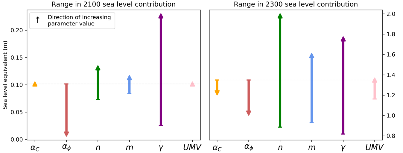
Figure 5. Sensitivity of Antarctic sea level contribution to each perturbed parameter at (a) 2100 and (b) 2300. Arrows denote the range in sea level contribution between ensemble members with minimal and maximal values of that parameter, pointing from minimal to maximal. Arrows pointing upwards/downwards therefore indicate a parameter that increases/decreases sea level contribution with higher values. The dashed horizontal line indicates the sea level contribution in a simulation with all parameters held at their default value.
