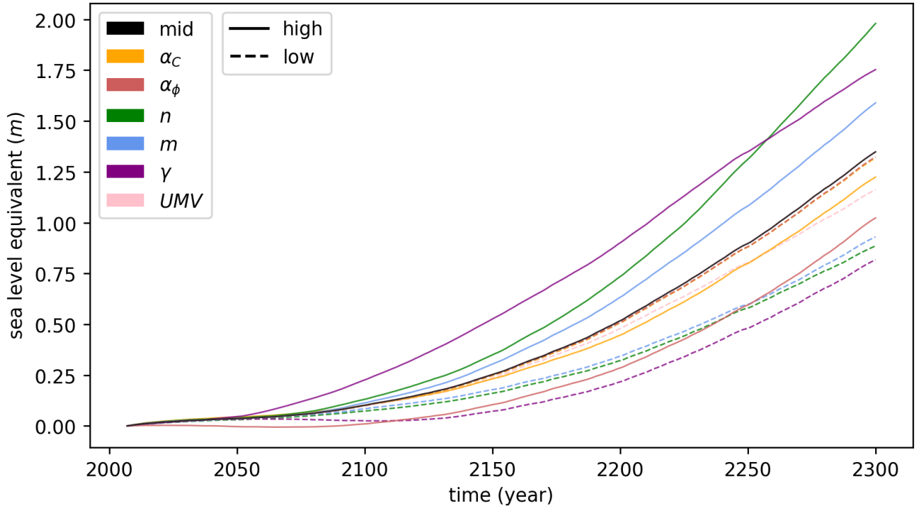
Figure 3. Timeseries of Antarctic sea level contribution for high and low values of each perturbed parameter.
