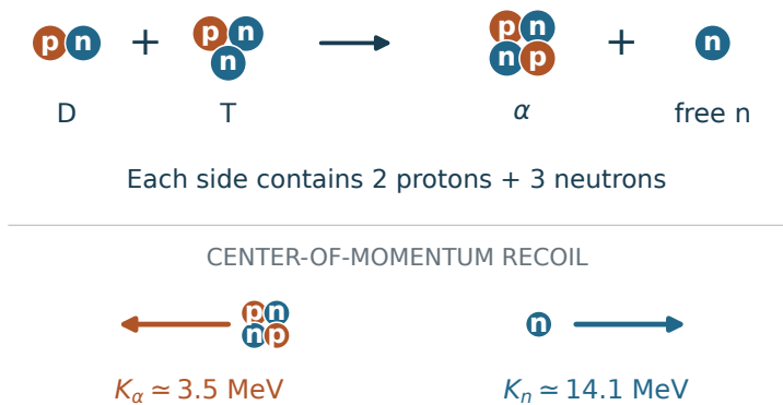
Figure 2: The same 2p+3n inventory is rearranged. The two final recoil arrows have equal momentum magnitude, not equal kinetic energy; energies use the leading nonrelativistic estimate in the text. Rest energies are measured relative to separated nucleons. Nucleon circles encode counts, not exact positions or nuclear shapes. Original diagram using sources 11 and 16 and Eq. (3).
