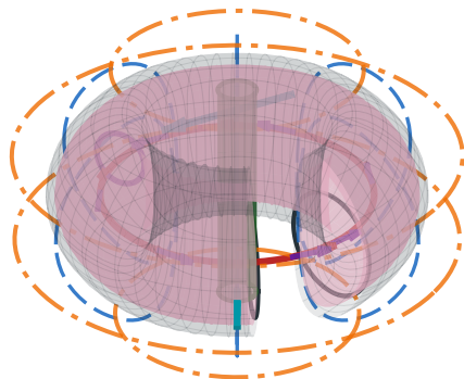
perspective view (vessel cut open)
