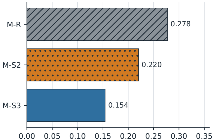
Trio (15,850 races)
