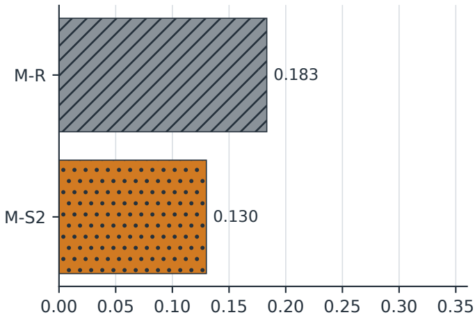
Quinella (19,269 races)
