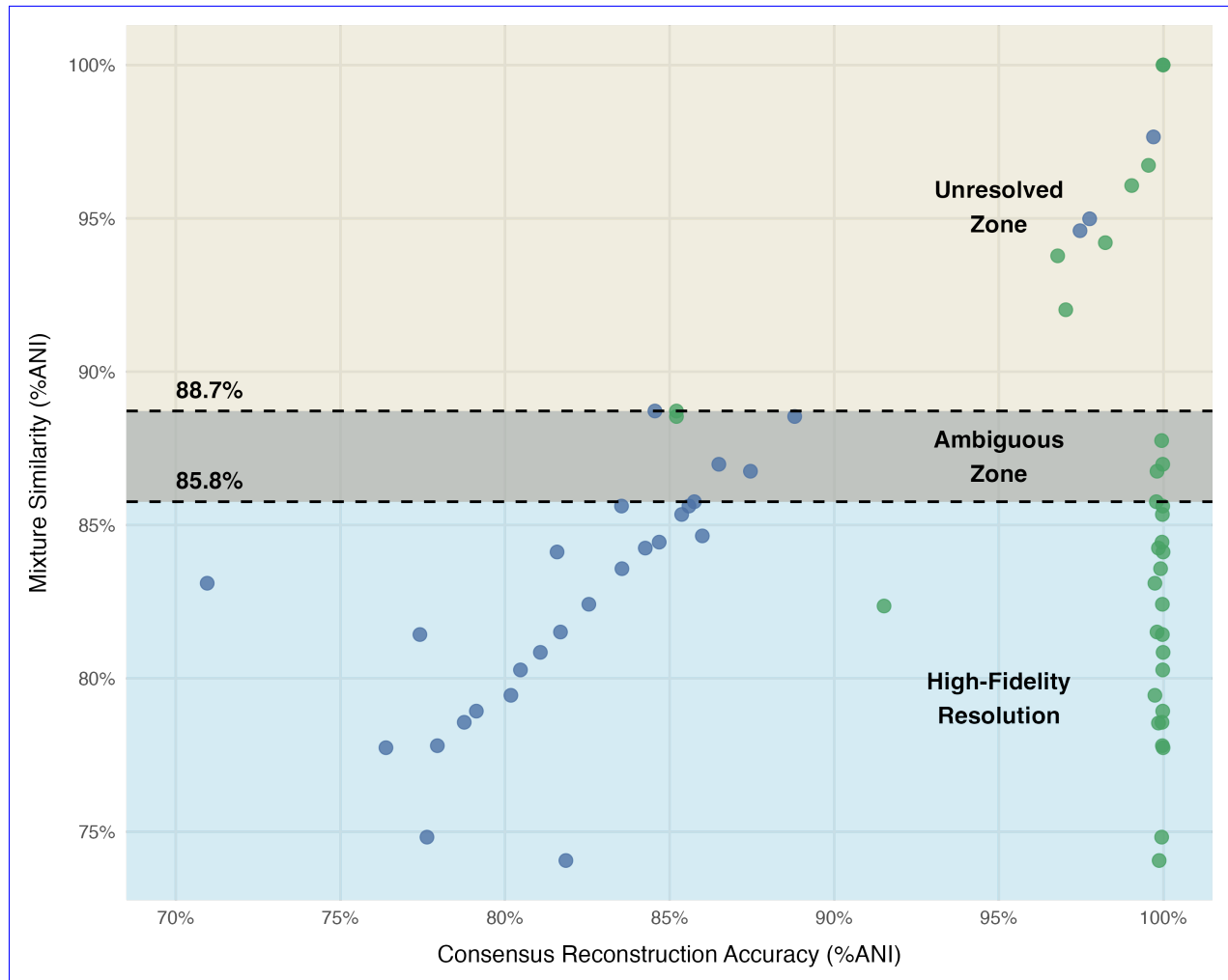
Figure 1: Mixture resolution dynamics across a genetic diversity gradient. This scatter plot characterises nf-core/viralmetagenome's ability to resolve coinfections of varying genetic similarity. The Y-axis represents the Average Nucleotide Identity (ANI) between the two target genomes present in the simulated mixture (Target vs. Representative), while the X-axis indicates the ANI of the reconstructed consensus genomes compared to the constant target genome.
