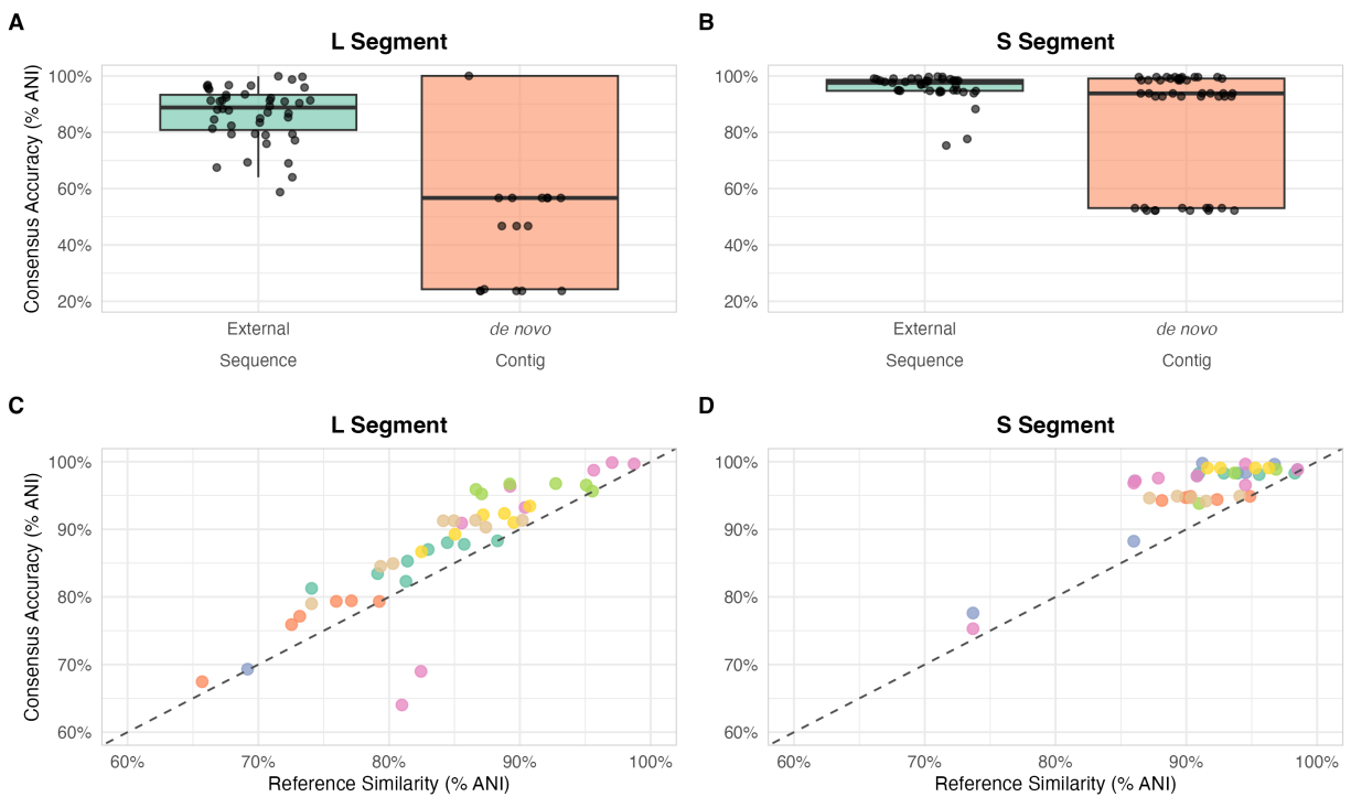
Figure 2: Impact of scaffolding reference similarity on consensus reconstruction accuracy (n=7 Lassa virus samples). The baseline consensus corresponds to the genome generated using the pipeline's automated reference selection from the complete U-RVDB reference pool. (A, B) Boxplots comparing consensus genome accuracy (ANI % relative to baseline) using external scaffolding reference sequences as versus de novo contigs alone for both L and S segments. For the high-coverage S segment, de novo contigs perform comparably to external references, whereas for the low-coverage L segment, external references significantly improve accuracy. (C, D) Scatter plots illustrating the relationship between scaffolding reference similarity (ANI % to baseline) and final consensus accuracy (ANI % to baseline) for L and S segments. The dashed line represents the line of identity ( y = x ), and points are colored by sample.
