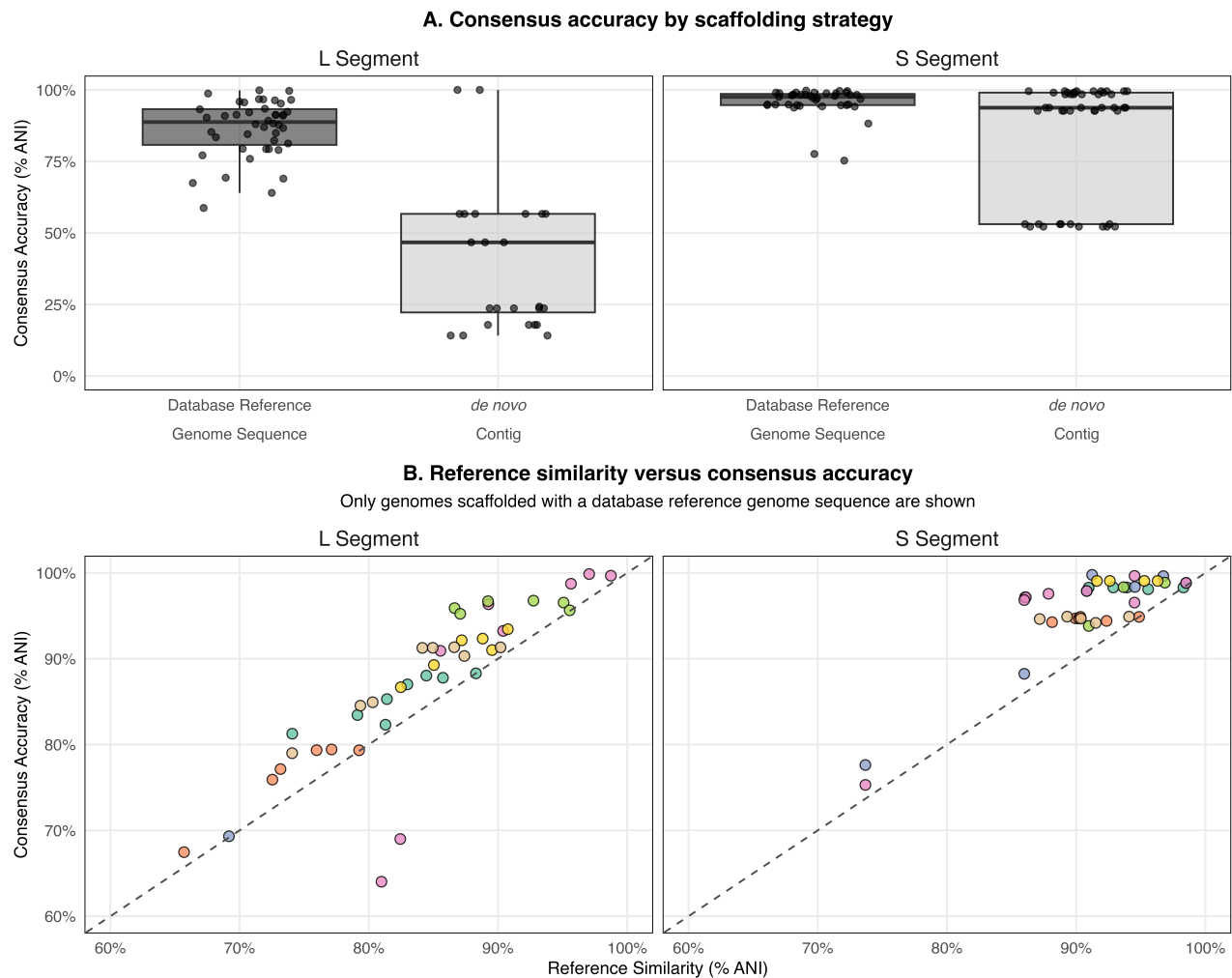
Fig. 4. Impact of scaffolding reference similarity on consensus reconstruction accuracy. Consensus accuracy is defined as the ANI (Eq. 1 in Supplementary Methods) between the test consensus and the baseline consensus (generated using the pipeline's automated reference selection from the full unclustered-RVDB). Test consensus genomes were scaffolded using either a supplied database reference genome or a de novo contig. (A) Boxplots comparing Consensus Accuracy (% ANI) for the L and S segments. The plots contrast the performance of using a database reference genome as the scaffolding backbone (dark grey) against relying solely on the de novo contig (light grey). For the low-coverage L segment, using the database reference genome significantly improves accuracy, whereas for the high-coverage S segment, the de novo route performs comparably to the database reference genome scaffolding (sequencing depths detailed in Figure 3). (B) Scatter plots illustrate the relationship between reference similarity and consensus accuracy (% ANI) for the L and S segments. Here, reference similarity is defined as the ANI between the supplied database reference genome sequence and the baseline consensus genome. The dashed line represents the line of identity ( y = x ), and points are coloured by sample source (Supplementary Fig. S1). Only consensus genomes that used a database reference genome sequence as the scaffold reference are shown in panel B.
