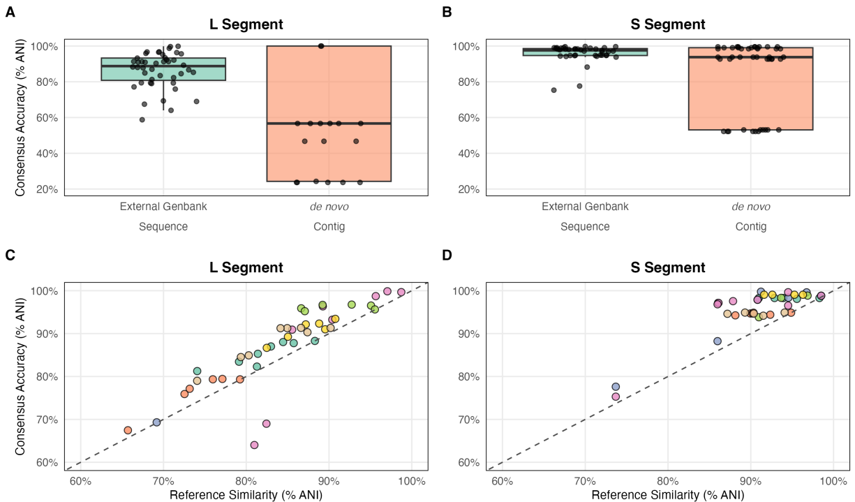
Figure 2: Impact of scaffolding reference similarity on consensus reconstruction accuracy. Consensus Accuracy is defined as the ANI between the test consensus (generated with a forced scaffolding reference) and the baseline consensus (generated using the pipeline’s automated reference selection from the full unclustered-RVDB). (A, B) Boxplots comparing Consensus Accuracy (% ANI) for the L and S segments. The plots contrast the performance of using an “external GenBank sequence” (green) as the scaffolding backbone against relying solely on “ de novo Contig” (orange). For the low-coverage L segment (A) , using GenBank references considerably improve accuracy, whereas for the high-coverage S segment (B) , the de novo contig performs comparable to reference scaffolding (sequencing depths detailed in Supplementary Figure S3). (C, D) Scatter plots illustrating the relationship between reference similarity (% ANI) and consensus accuracy (% ANI). The dashed line represents the line of identity ( y = x ), and points are colored by sample source (as per Supplementary Figure 2). Note: only consensus genomes that used a GenBank sequence as scaffold reference are plotted in C and D.
