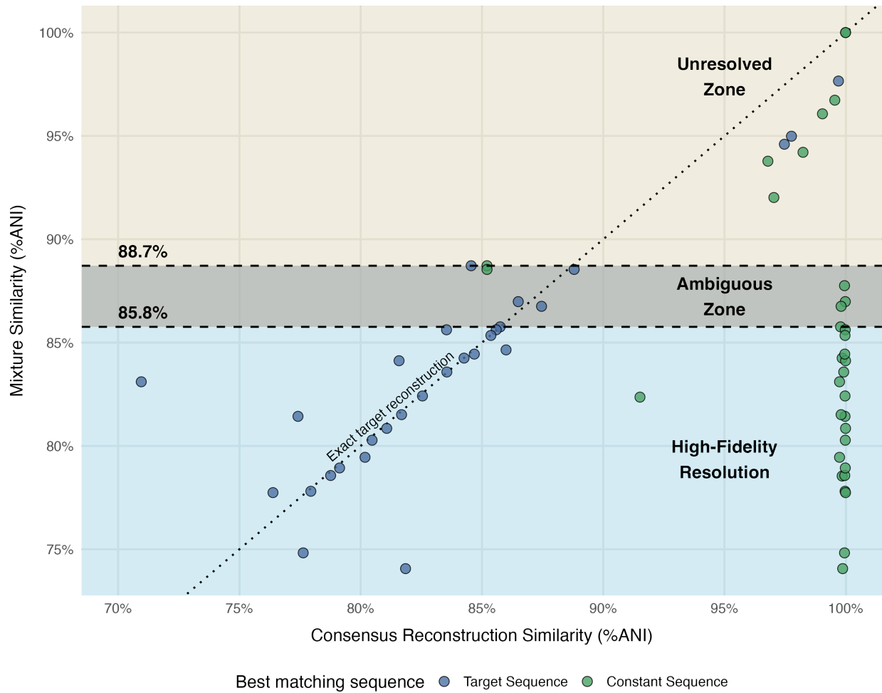
Supplementary Fig. S1: Mixture resolution dynamics across a genetic diversity gradient. This scatter plot characterises nf-core/viralmetagenome 23 's ability to resolve co-infections of varying genetic similarity. The Y-axis (Mixture Similarity) represents the Average Nucleotide Identity (ANI (approximate matches; Eq. 1) between the two target-reference genomes present in the simulated mixture ( Target -target genome vs. Representative constant representative MN090277.1); while the . The X-axis (Consensus Reconstruction Similarity) indicates the ANI (approximate matches) of the reconstructed consensus genomes compared to the constant target-reference genome MN090277.1. Green dots are consensus genomes most similar to the constant reference genome; blue dots represent consensus genomes with best matches towards the target sequence. Successful mixture separation is indicated by a blue dot on the diagonal and a green dot at 100% reconstruction similarity. Three empirically determined zones are highlighted: Unresolved (>88.7% mixture similarity), Ambiguous (85.8–88.7%), and High-Fidelity Resolution (<85.8%).
