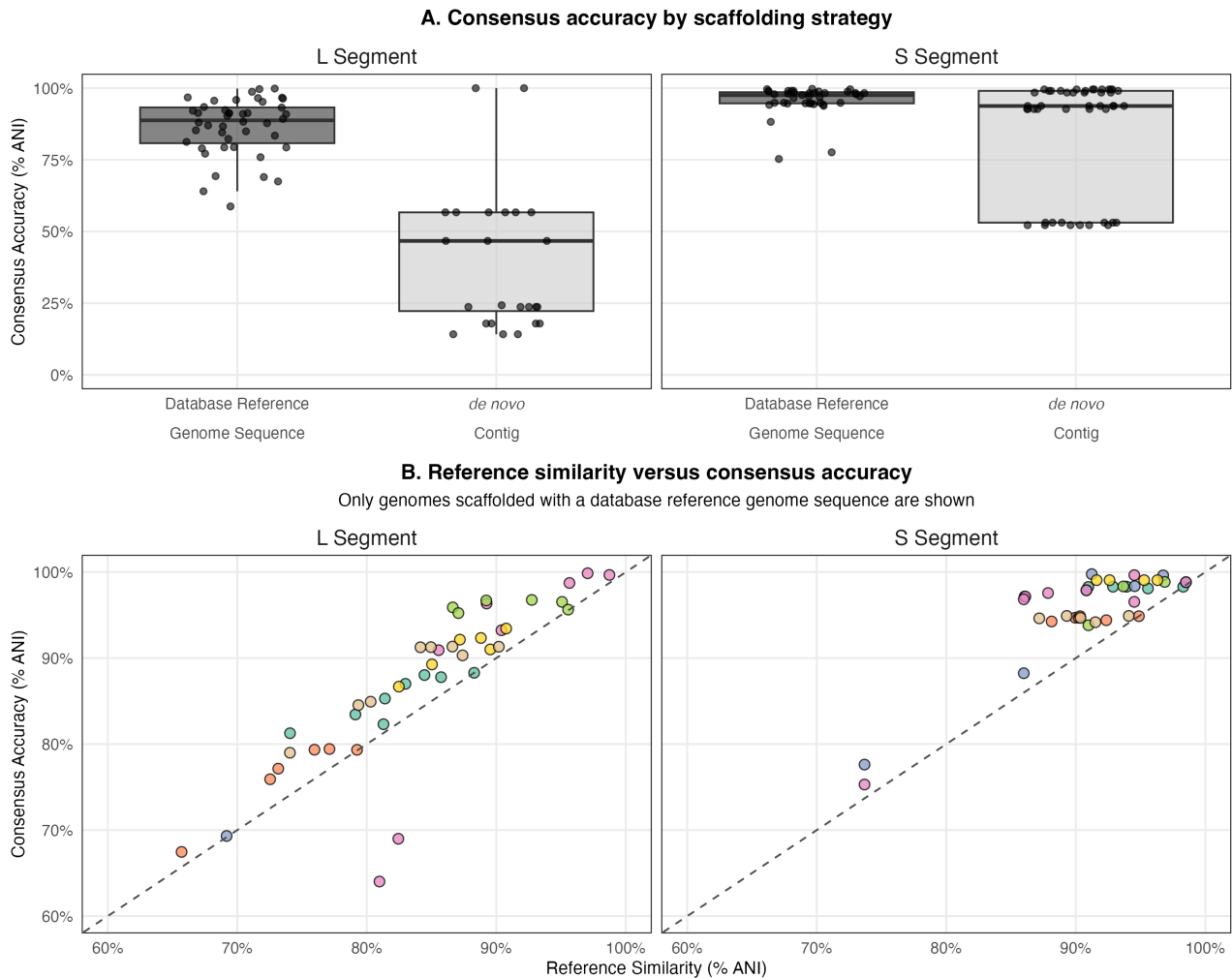
Fig. 2. Impact of scaffolding reference similarity on consensus reconstruction accuracy. Consensus accuracy is defined as the ANI between the test consensus and the baseline consensus (generated using the pipeline's automated reference selection from the full unclustered-RVDB). Test consensus genomes were scaffolded using either a supplied database reference genome or a de novo contig. (A) Boxplots comparing Consensus Accuracy (% ANI) for the L and S segments. The plots contrast the performance of using a database reference genome as the scaffolding backbone (dark grey) against relying solely on the de novo contig (light grey). For the low-coverage L segment, using the database reference genome sequences significantly improves accuracy, whereas for the high-coverage S segment, the de novo route performs comparable to the database reference genome scaffolding (sequencing depths detailed in Supplementary Figure S3). (B) Scatter plots illustrate the relationship between reference similarity and consensus accuracy (% ANI) for the L and S segments. Here, reference similarity is defined as the ANI between the supplied database reference genome sequence and the baseline consensus genome. The dashed line represents the line of identity ( y = x ), and points are coloured by sample source (Supplementary Figure S2). Only consensus genomes that used a database reference genome sequence as the scaffold reference are shown in panel B.
