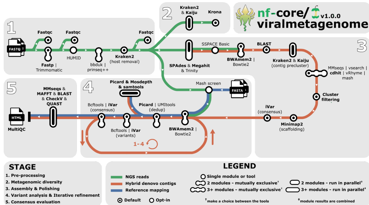
Figure 1: Overview of the nf-core/viralmetagatome pipeline for untargeted viral genome reconstruction. Default options are highlighted in bold. nf-core/viralmetagatome processes short-read data through pre-processing, metagenomic diversity assessment, de novo assembly with multiple assemblers, scaffolding with automated reference identification and taxonomy-guided clustering of contigs, and iterative consensus refinement through read mapping and consensus calling. Quality control metrics, assembly statistics, and coverage data are integrated into interactive MultiQC reports and standardised overview tables for downstream analysis.
