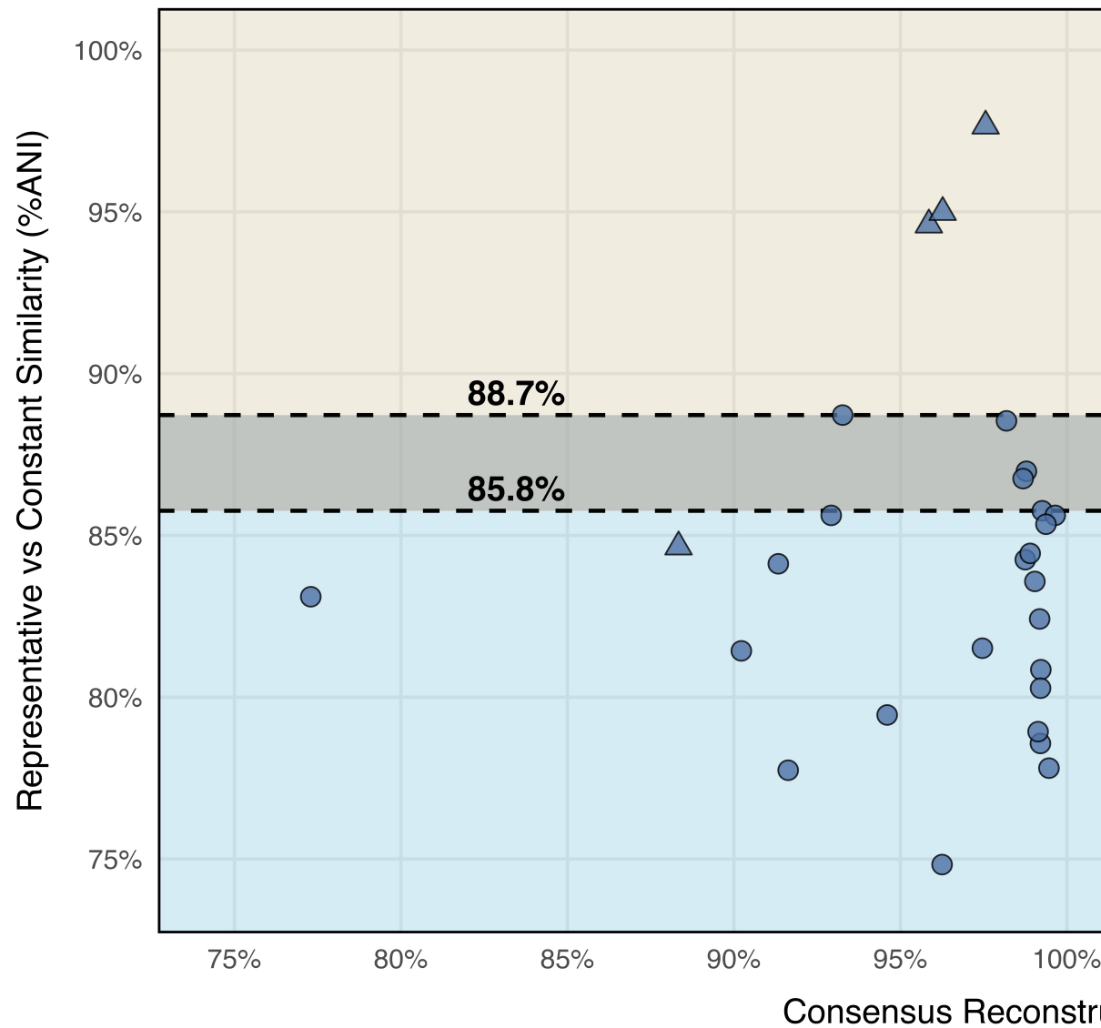
Representative genome
