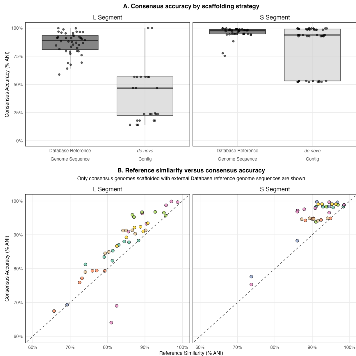
Figure 2: Impact of scaffolding reference similarity on consensus reconstruction accuracy. Consensus accuracy is defined as the ANI between the test consensus (generated with a forced scaffolding reference) and the baseline consensus (generated using the pipeline’s automated reference selection from the full unclustered-RVDB). (A) Boxplots compare consensus accuracy (% ANI) for the L and S segments, contrasting use of a database reference genome sequence (green) as the scaffolding backbone against relying solely on the “ de novo contig” (orange). For the low-coverage L segment, the database reference genome sequence considerably improves accuracy, whereas for the high-coverage S segment, the de novo contig performs comparably to reference scaffolding (sequencing depths detailed in Supplementary Figure S3). (B) Scatter plots illustrate the relationship between reference similarity and consensus accuracy (% ANI) for the L and S segments. Here, reference similarity is defined as the ANI between the supplied database reference genome sequence and the baseline consensus genome. The dashed line represents the line of identity ( y = x ), and points are coloured by sample source (Supplementary Figure S2). Only consensus genomes that used a database reference genome sequence as the scaffold reference are shown in panel B.
