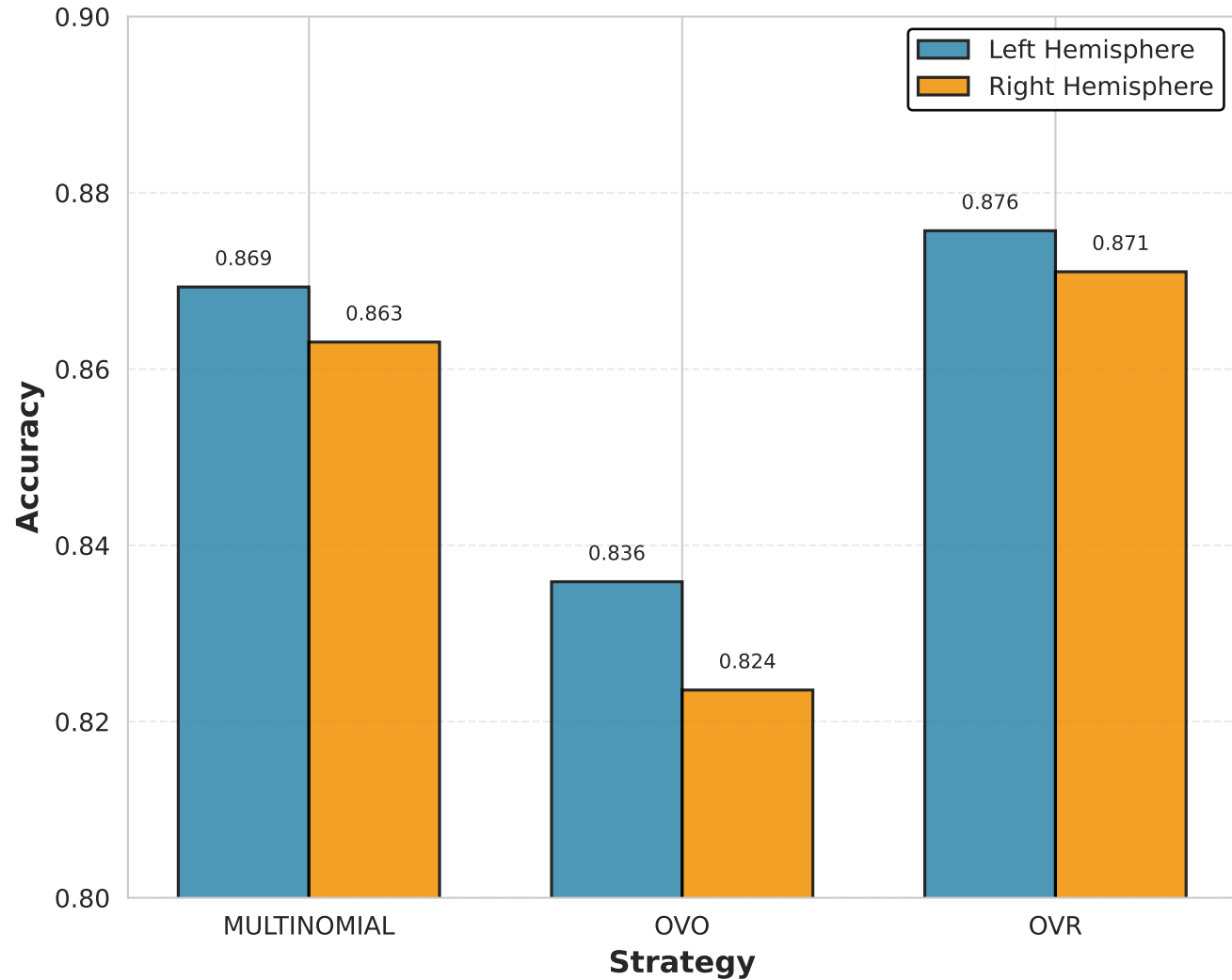
B) Task Performance: Left vs Right Hemisphere
