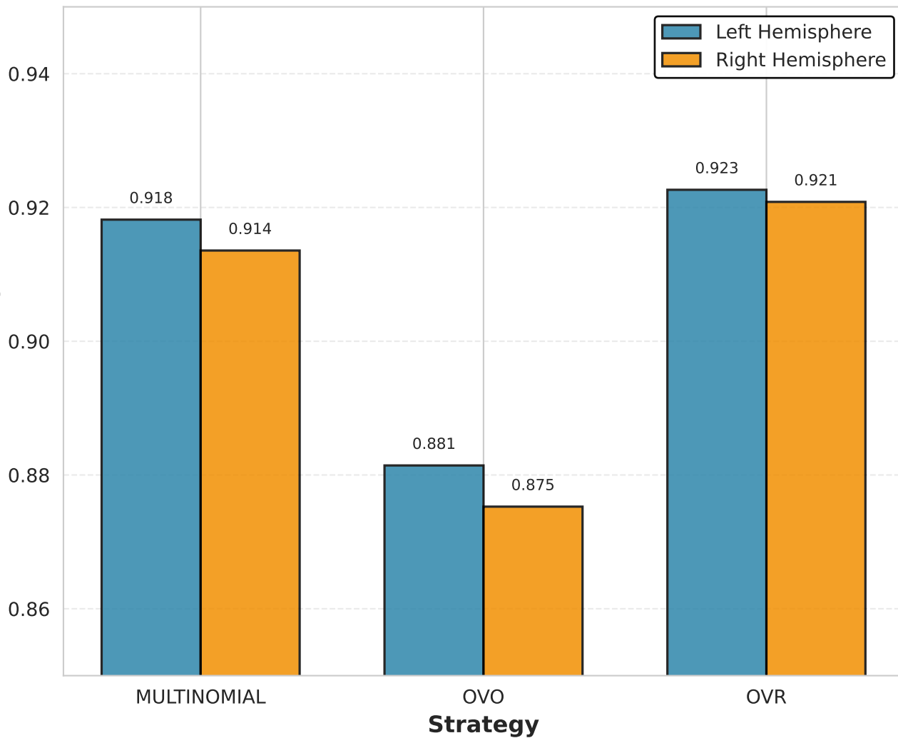
A) CV Performance: Left vs Right Hemisphere
