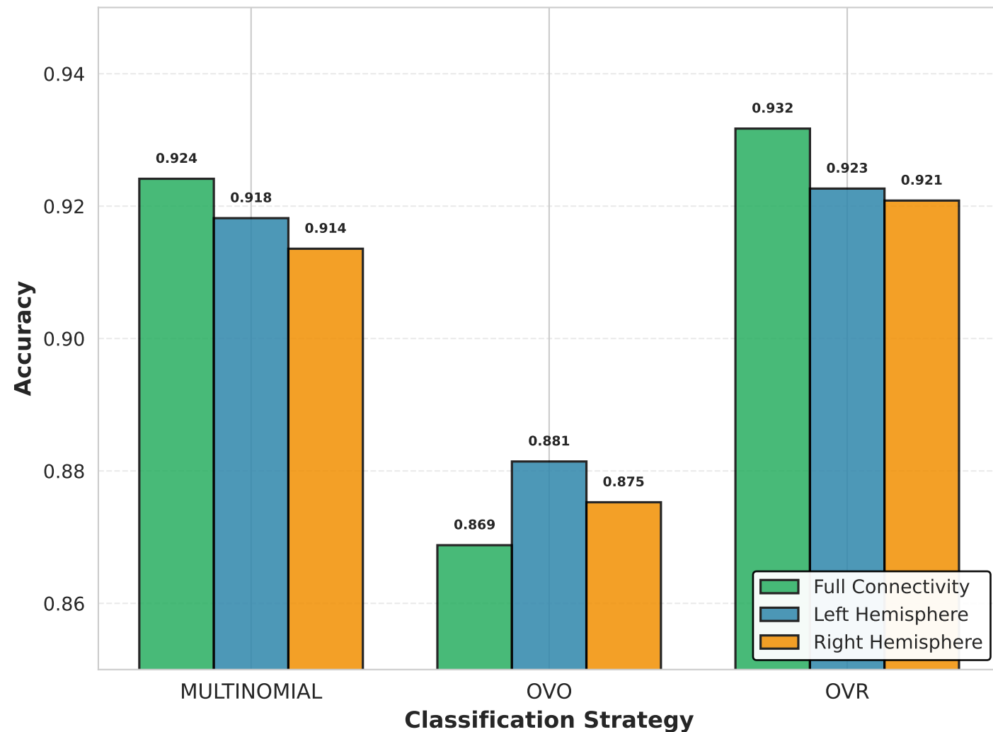
A) CV Performance: Full vs Hemisphere Analysis
