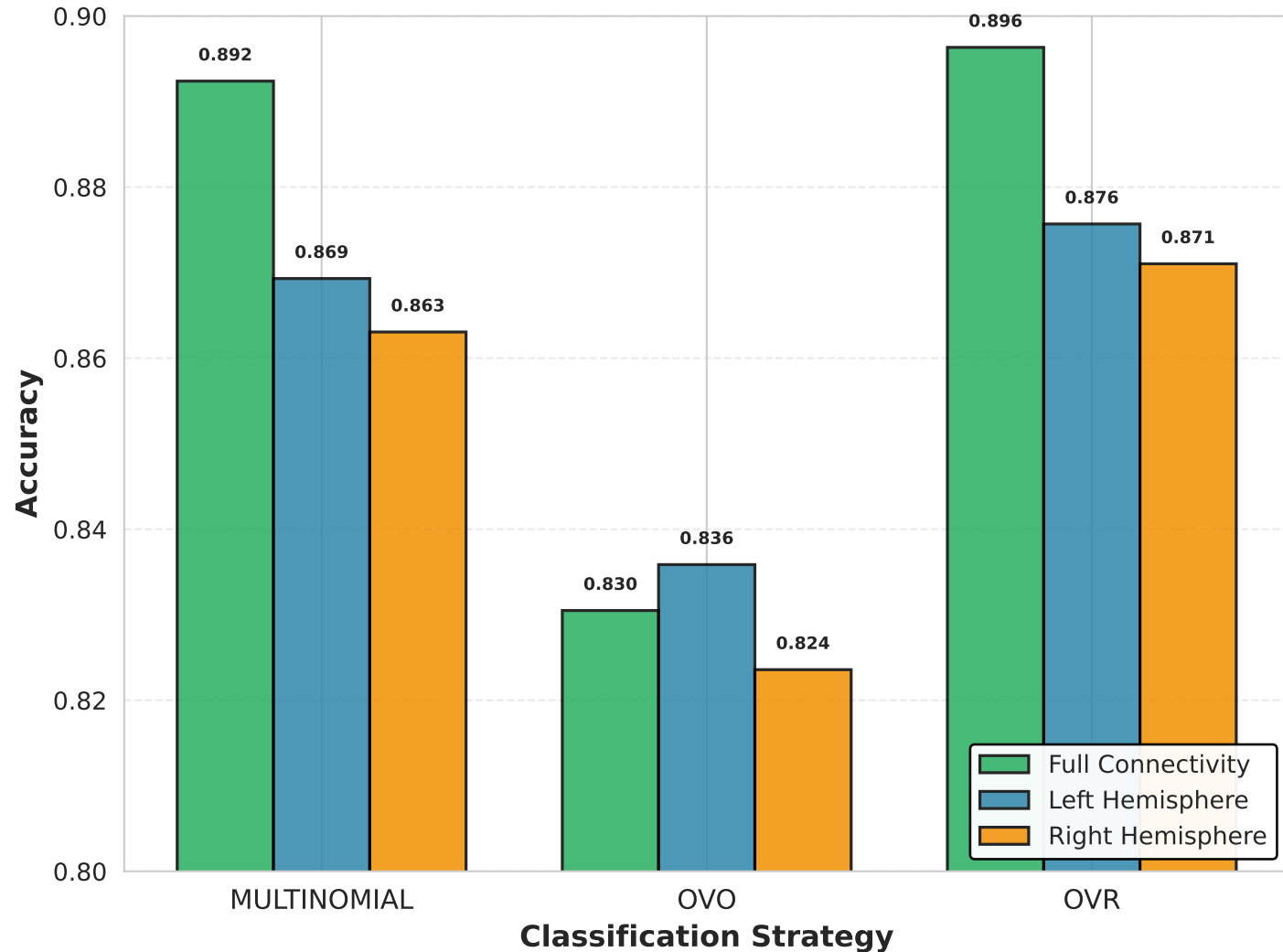
B) Task Performance: Full vs Hemisphere Analysis
