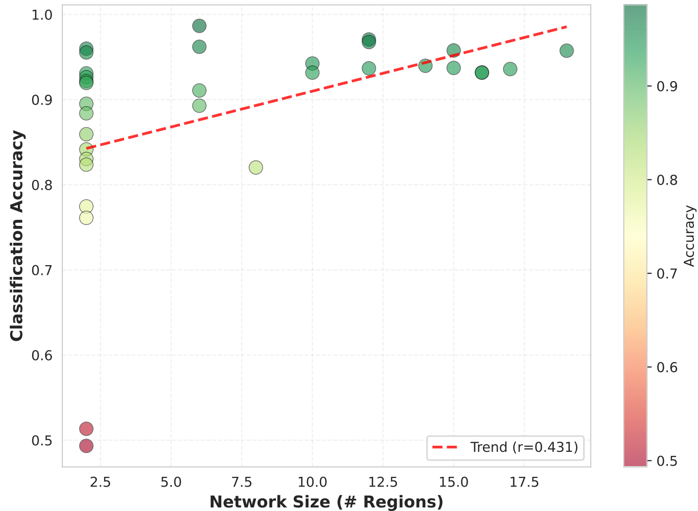
A) Network Size vs Classification Performance
