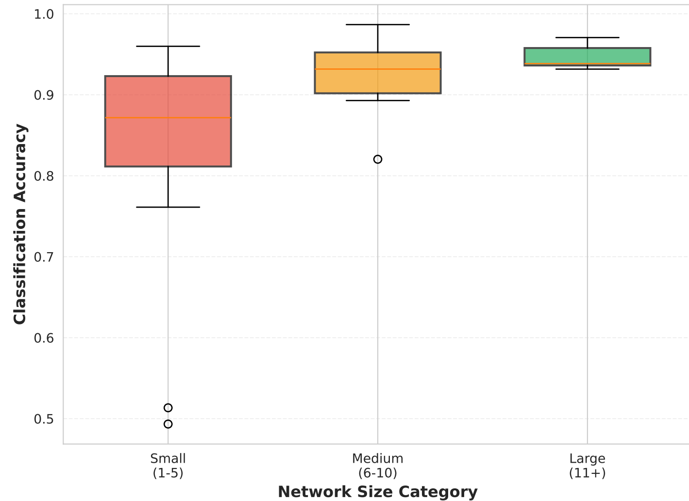
B) Performance Distribution by Network Size
