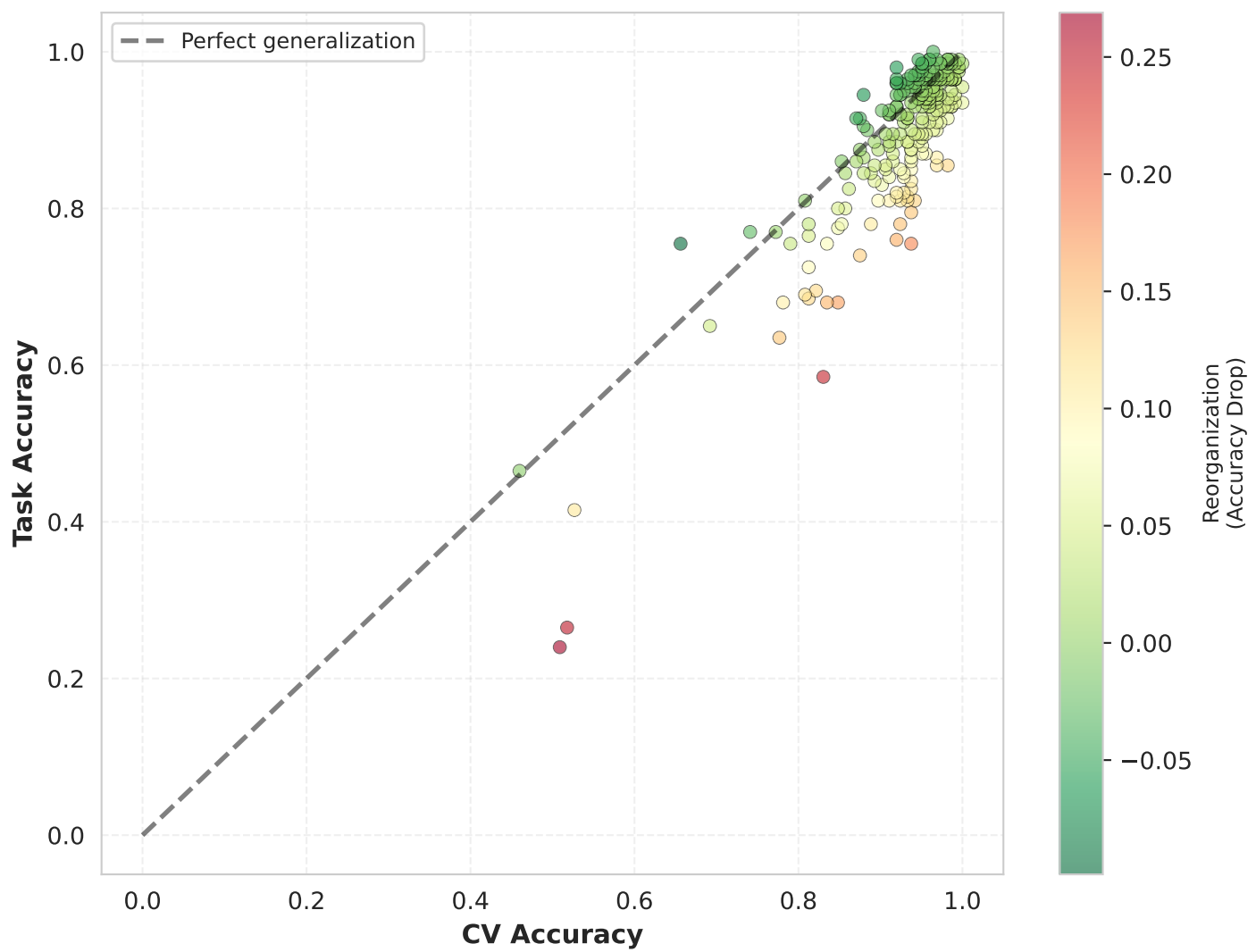
D) CV vs Task Performance by Region
