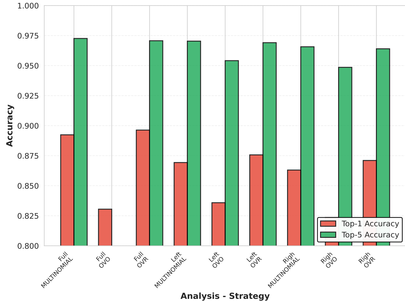
B) Task: Top-1 vs Top-5 Accuracy
