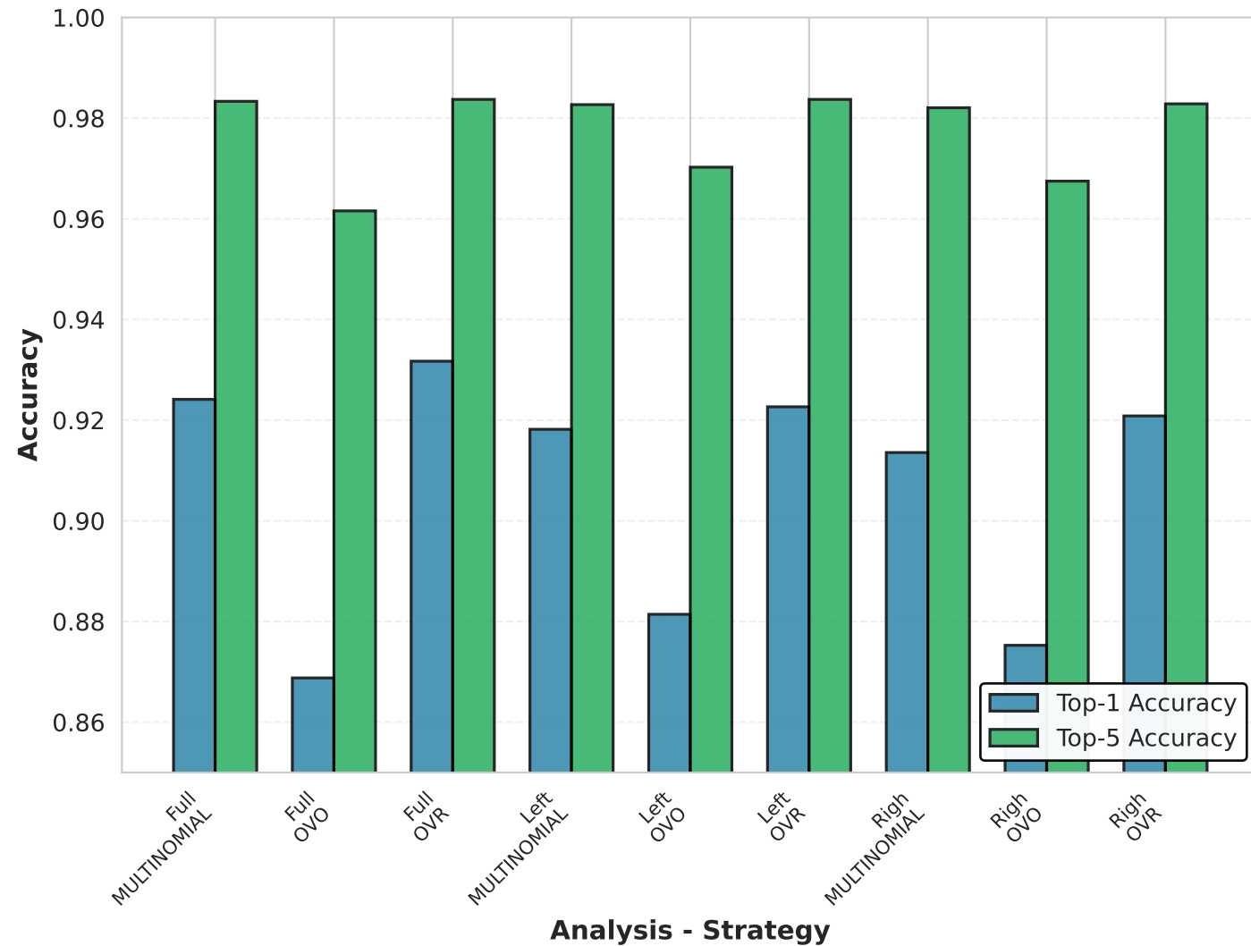
A) CV: Top-1 vs Top-5 Accuracy
