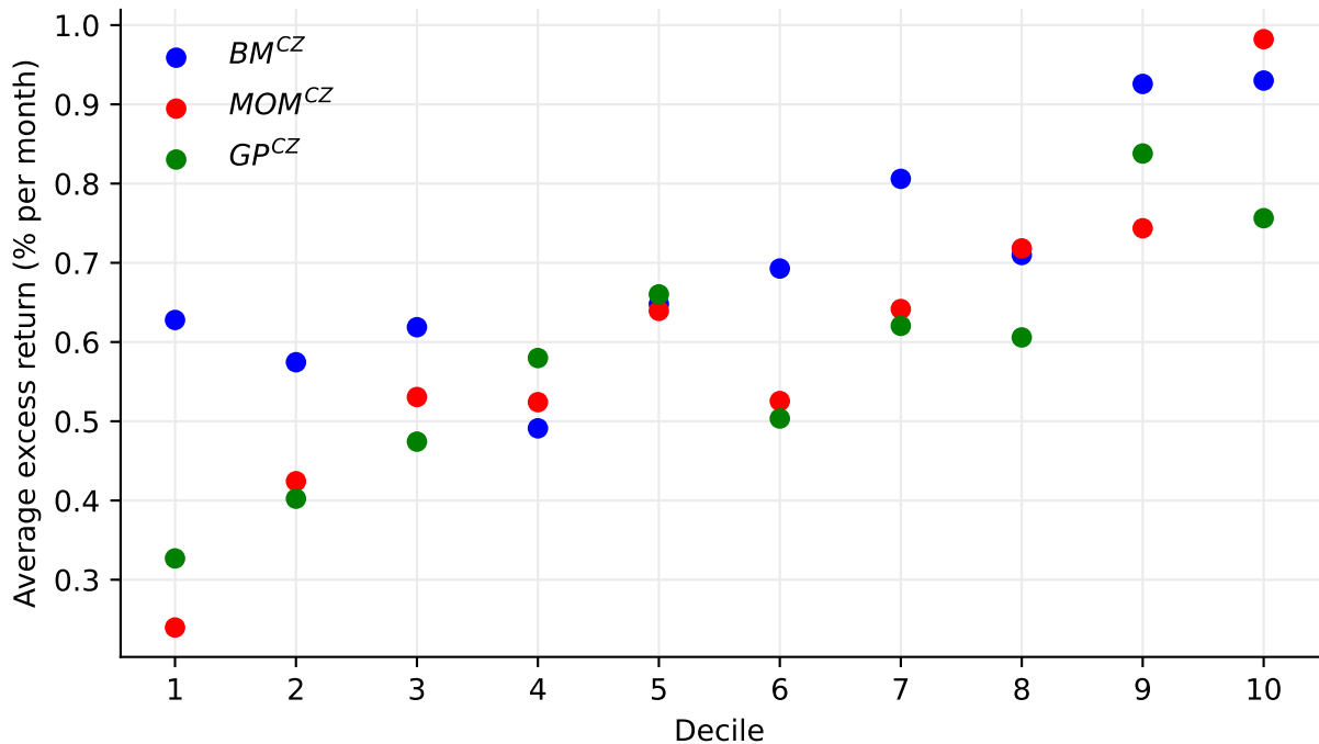
(iv) VW, annual rebalancing, general breakpoints
