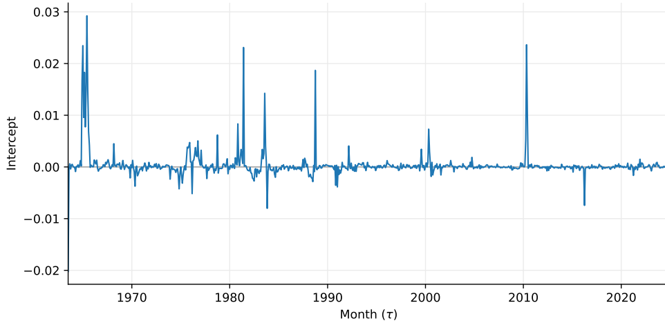
Figure 7: Intercept \hat{a}_\tau of the monthly cross-firm regression (23), 1963:06–2024:12. The grey line marks 0.
