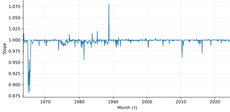
Figure 8: Slope \hat{b}_\tau of the monthly cross-firm regression (23), 1963:06–2024:12. The grey line marks 1.
