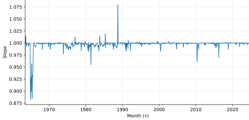
Figure 9: Slope \hat{b}_\tau of the monthly cross-firm regression (26), 1963:06–2024:12. The grey line marks 1.
