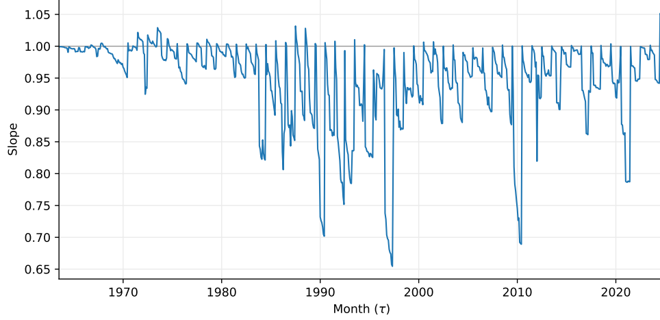
Figure 12: Slope \hat{b}_\tau of the monthly cross-firm regression (28), 1963:06–2024:12. The grey line marks 1.
