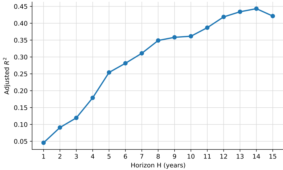
Figure 3: Adjusted R^2 of regression (17) against the horizon H (in years). Monthly observations, 1927:12–2021:12.
