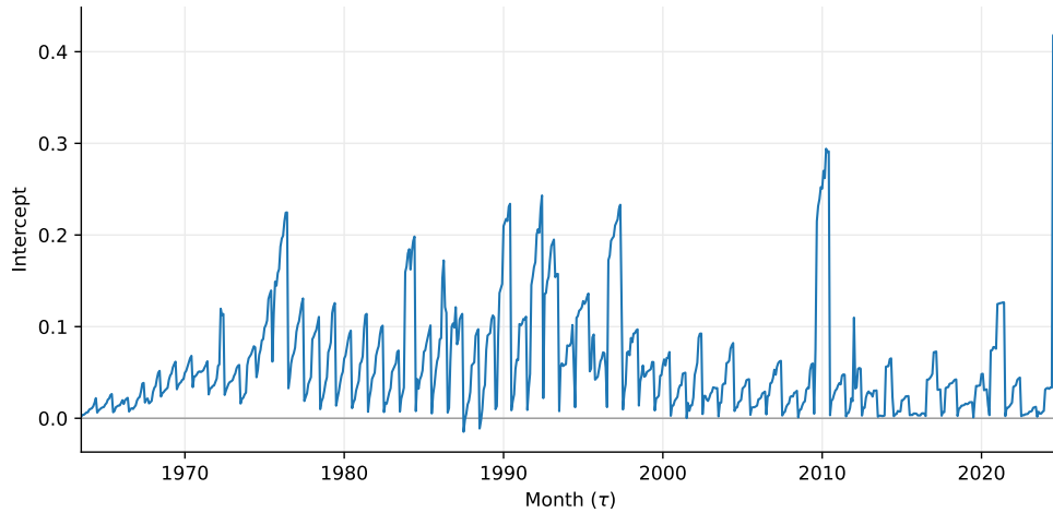
Figure 11: Intercept \hat{a}_\tau of the monthly cross-firm regression (28), 1963:06–2024:12. The grey line marks 0.
