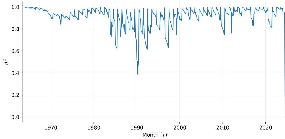
Figure 13: R^2 of the monthly cross-firm regression (28), 1963:06–2024:12. The grey line marks 1.
