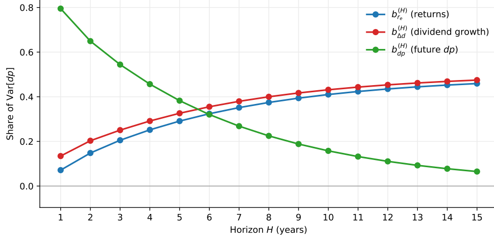
Figure 2: VAR-implied coefficients b_{re}^{(H)} , b_{\Delta d}^{(H)} and b_{dp}^{(H)} of (16) against the horizon H (in years), with \kappa = 0.9642 . VAR (14)–(15) with a 12-month step, estimated by OLS on monthly observations, 1927:12–2021:12.
