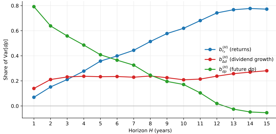
Figure 1: Coefficients b_{r_e}^{(H)} , b_{\Delta d}^{(H)} and b_{dp}^{(H)} of the decomposition (13) against the horizon H (in years), estimated on the EQ Dataset with \kappa = 0.9642 . Monthly observations, 1927:12–2021:12.
