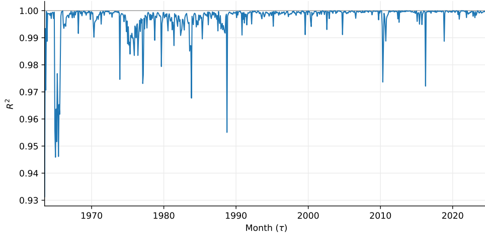
Figure 10: R^2 of the monthly cross-firm regression (38), 1963:06–2024:12. The grey line marks 1.
