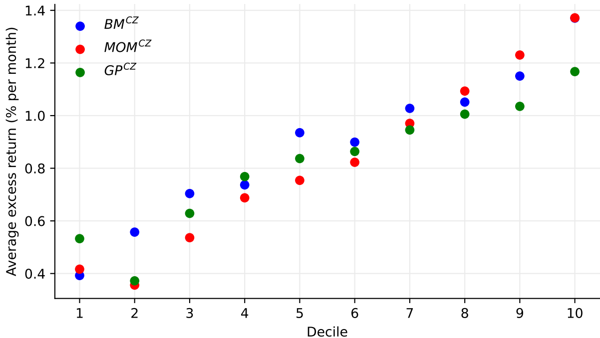
(v) EW, monthly rebalancing, general breakpoints
