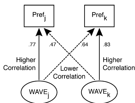
Fig. 2. Diagram showing a central tenet of the EVT: The correlation between WAVEs and color preferences obtained within a group should be stronger than the correlation between WAVEs and color preferences obtained from different groups. The correlations are obtained from individuals with similar color preferences as determined by hierarchical clustering (21). (Fig. S1 shows plots of the color preferences and WAVEs of these two groups.)
