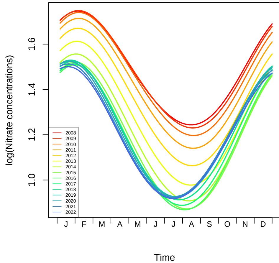
0.9 th expectile curve at Segment 87
