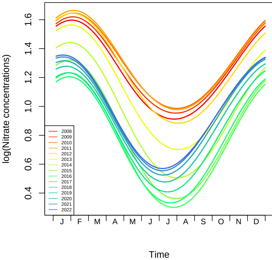
0.5 th expectile curve at Segment 87
