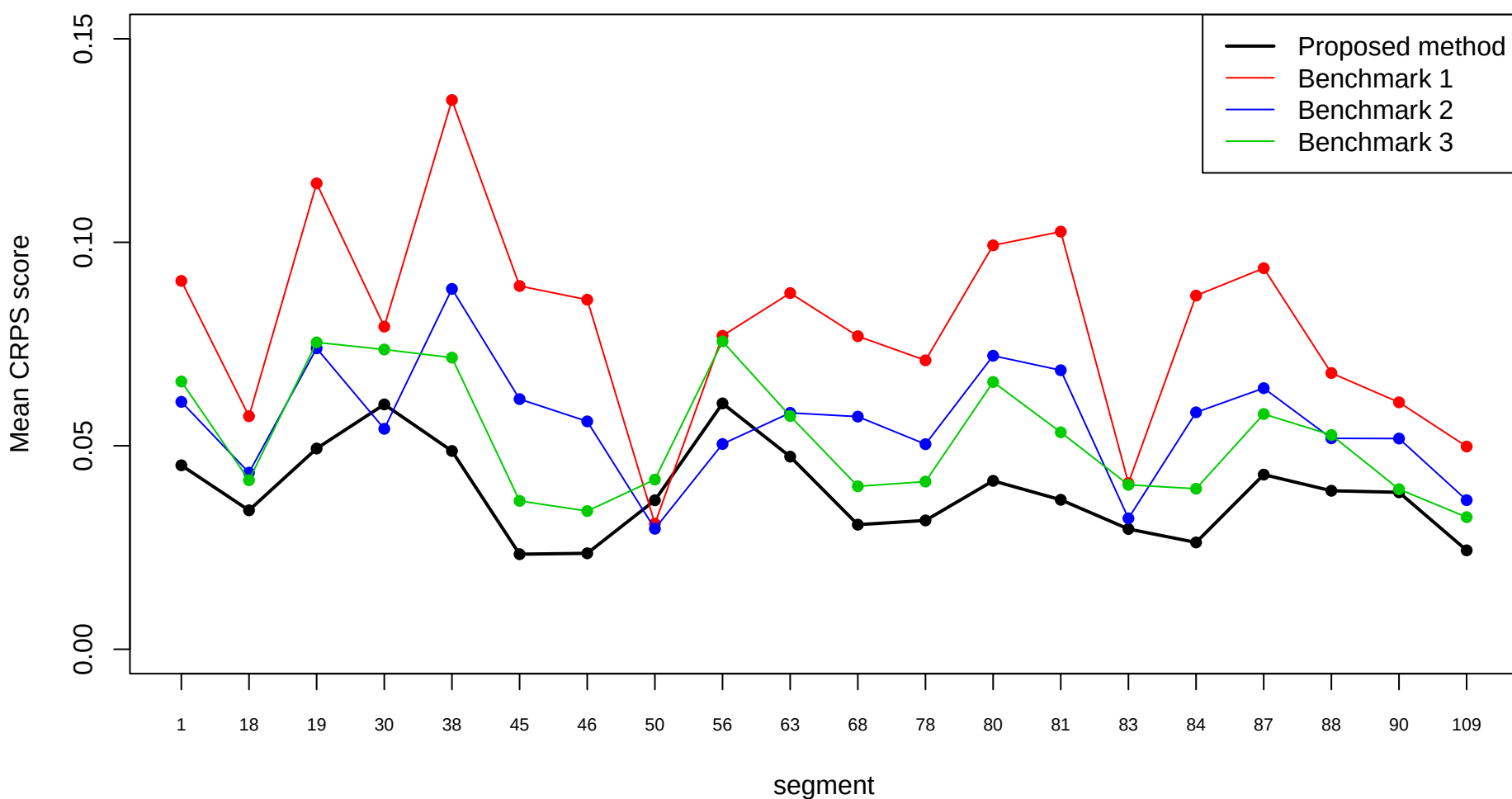
Average CRPS score for 1-year-ahead prediction
