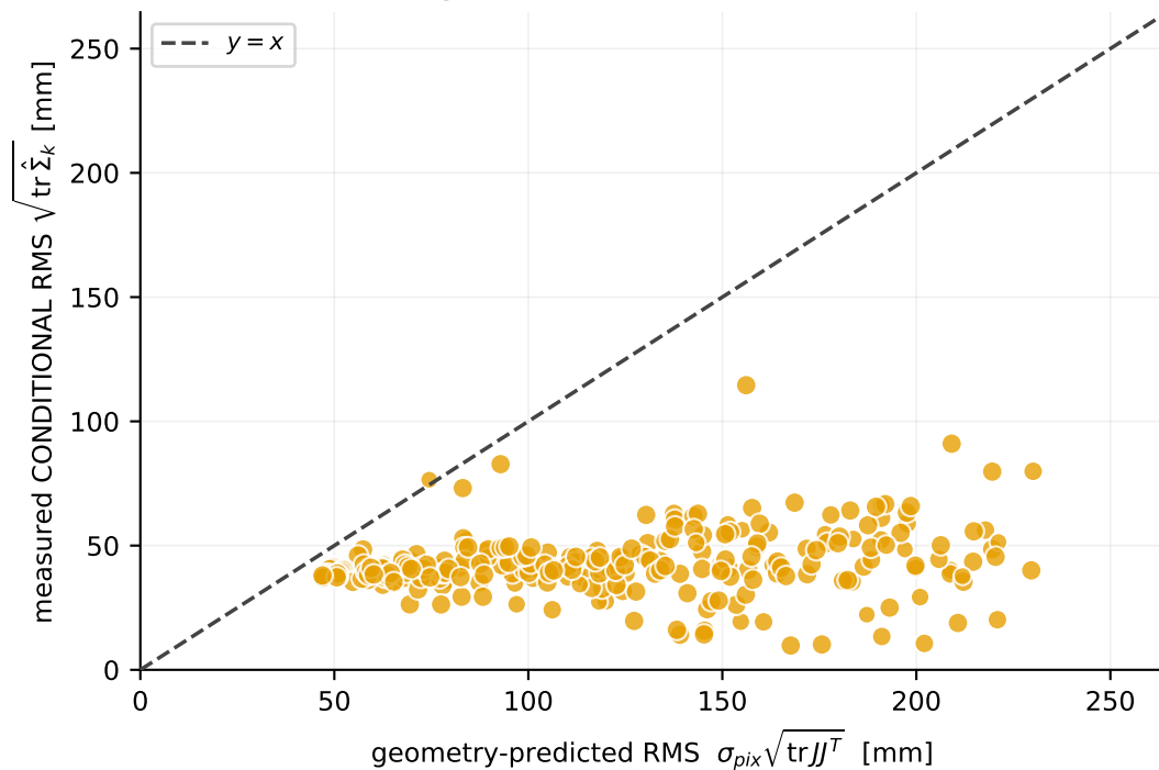
(b) does geometry predict the local SPREAD? N = 2320 detections · M = 284 cells (0.5 m, ≥ 5 each) conditional: R^2 vs identity = -54.22 · cell Spearman = +0.28 · median obs/pred = 0.38 median per-cell BIAS removed first = 70 mm
