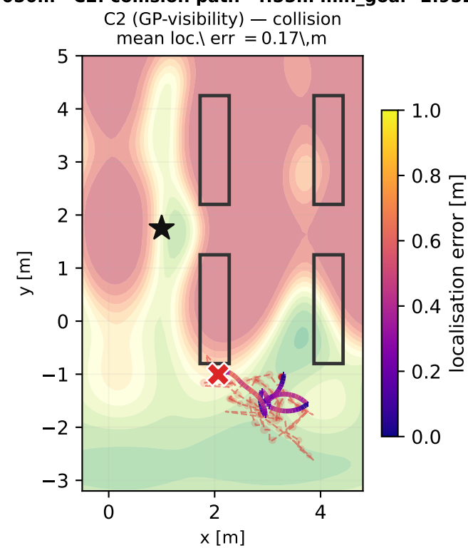
F38 — waypoint_radius=0.10 + sequential YOLO velocity correction C1: collision path=11.42m min_goal=2.050m C2: collision path=4.55m min_goal=2.952m
