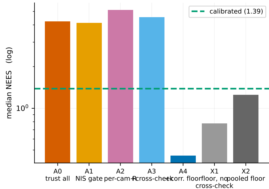
Is the stated uncertainty honest? above the line = overconfident
