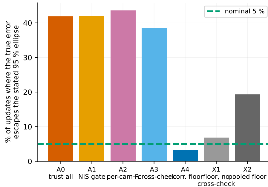
Unearned confidence (this is what drives into shelves)
