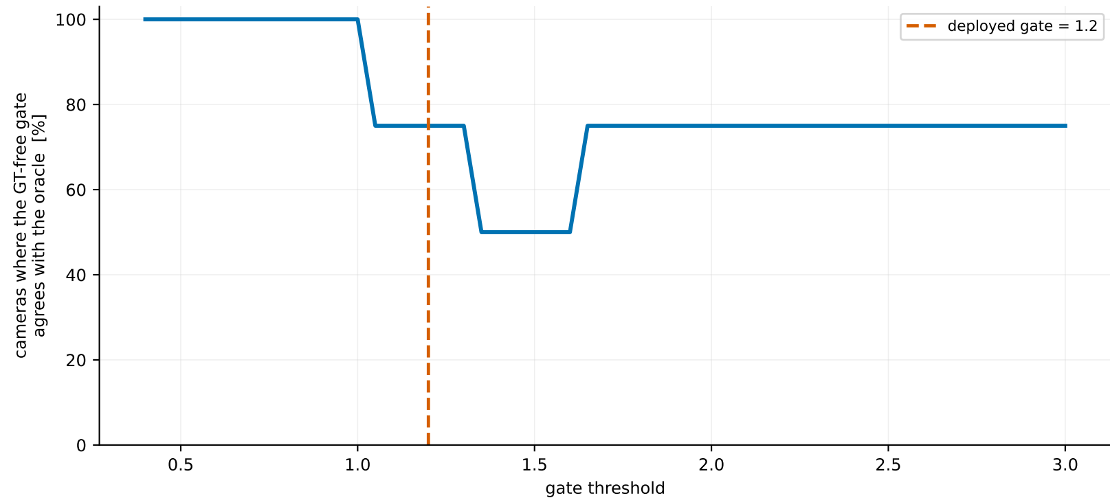
Threshold sensitivity of the deployable gate
