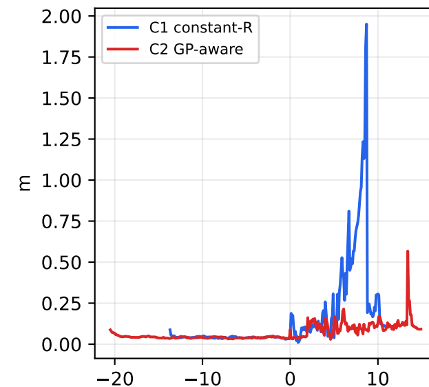
Planner belief error vs truth
