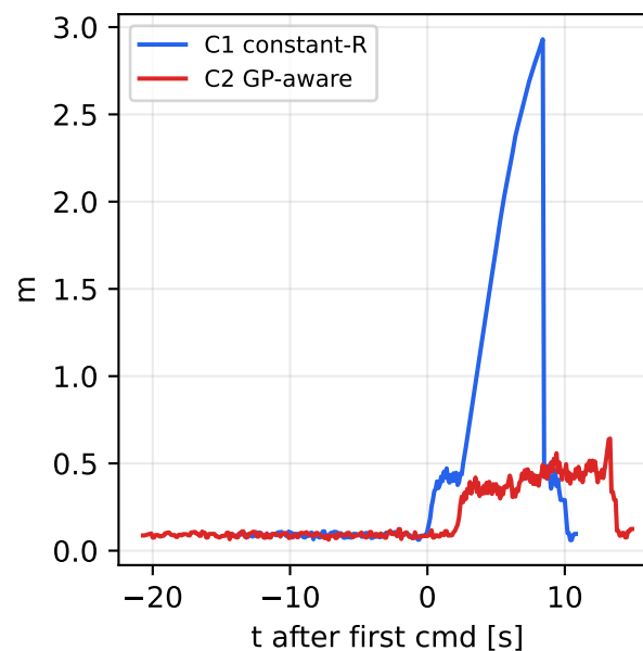
External-camera state error vs truth
