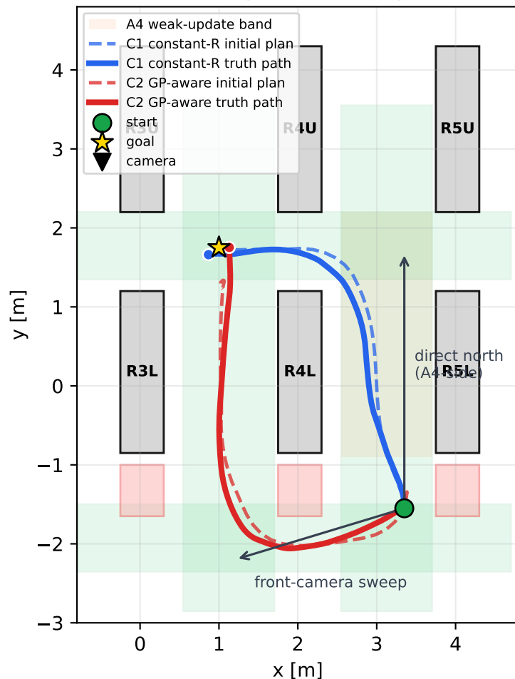
Boxside route-choice probe: initial plan vs execution
