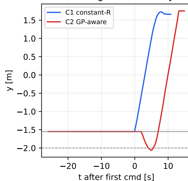
Route signature: truth y
