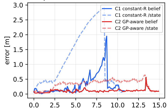
Truth error: planner belief vs external-camera state
