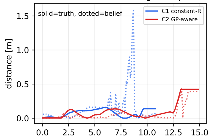
Deviation from initial global plan
