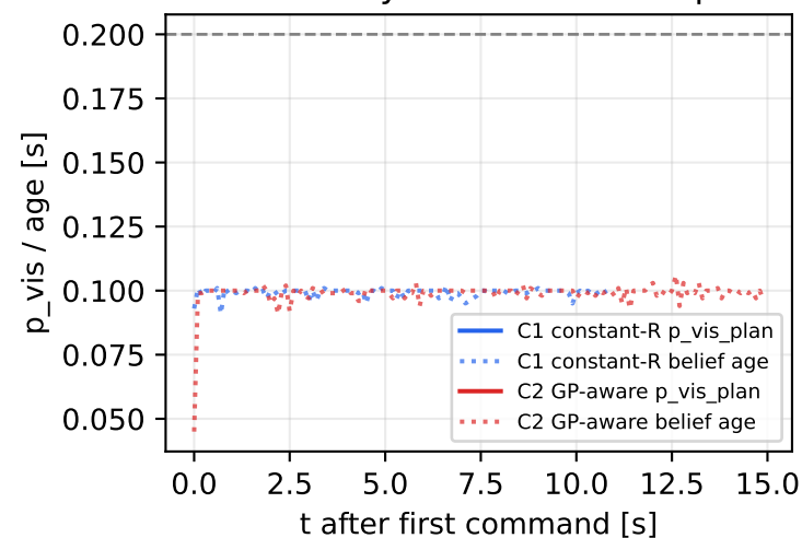
Planner visibility and stale-belief pressure
