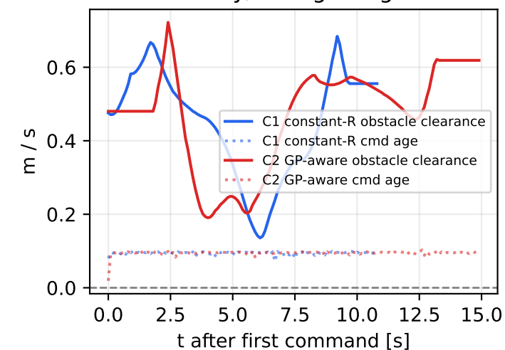
Safety/timing margin
