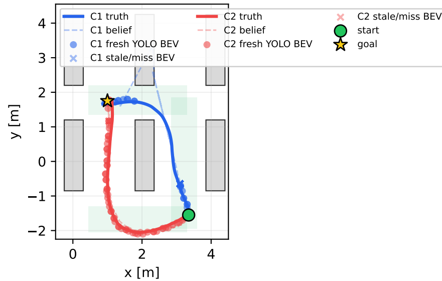
C2: perception and belief error while driving
