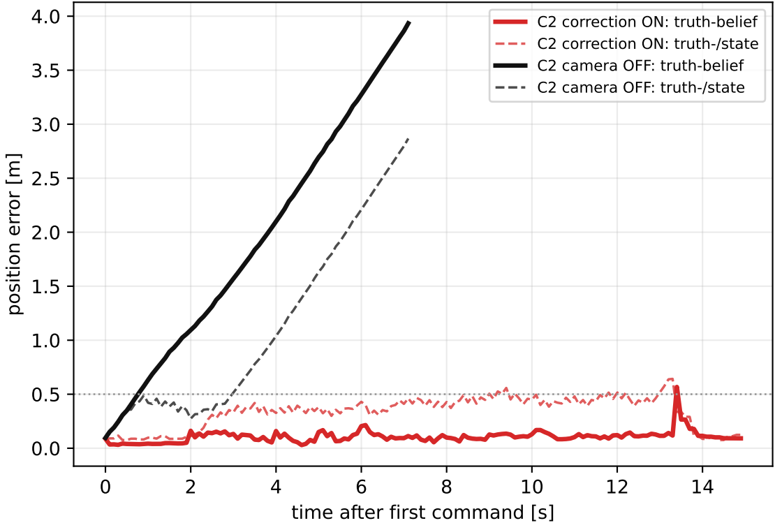
(b) Camera OFF: belief error explodes while correction ON stays bounded
