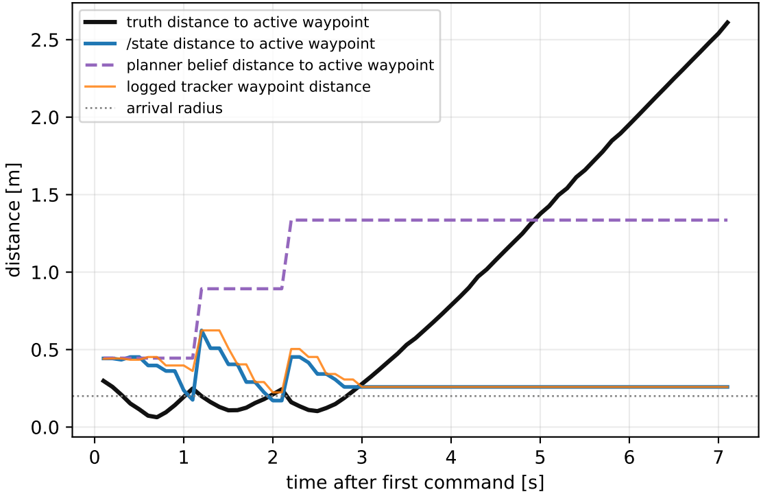
(c) Exact failure: tracker thinks stale /state is near waypoint 2
