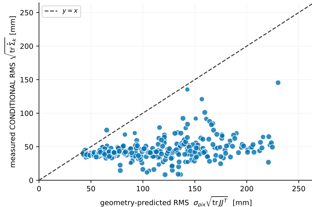
(b) does geometry predict the local SPREAD? N = 2556 detections · M = 316 cells (0.5 m, \geq 5 each) conditional: R^2 vs identity = -23.89 · cell Spearman = +0.36 · median obs/pred = 0.44 median per-cell BIAS removed first = 47 mm
