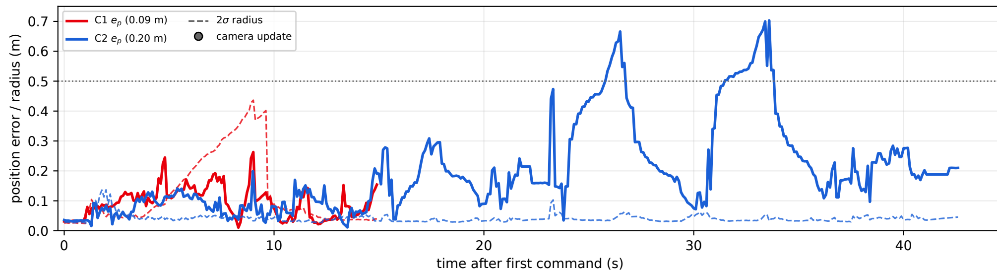
(c) Truth--belief error with 2\sigma belief radius
