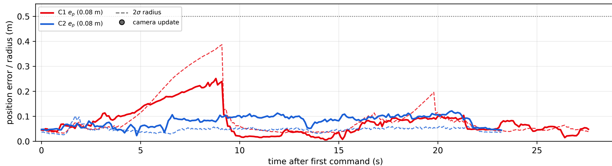
(c) Ground-truth belief error with 2σ belief radius
