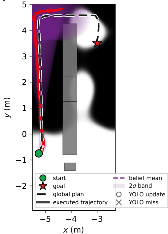
(a) Current C1: west lane failure
