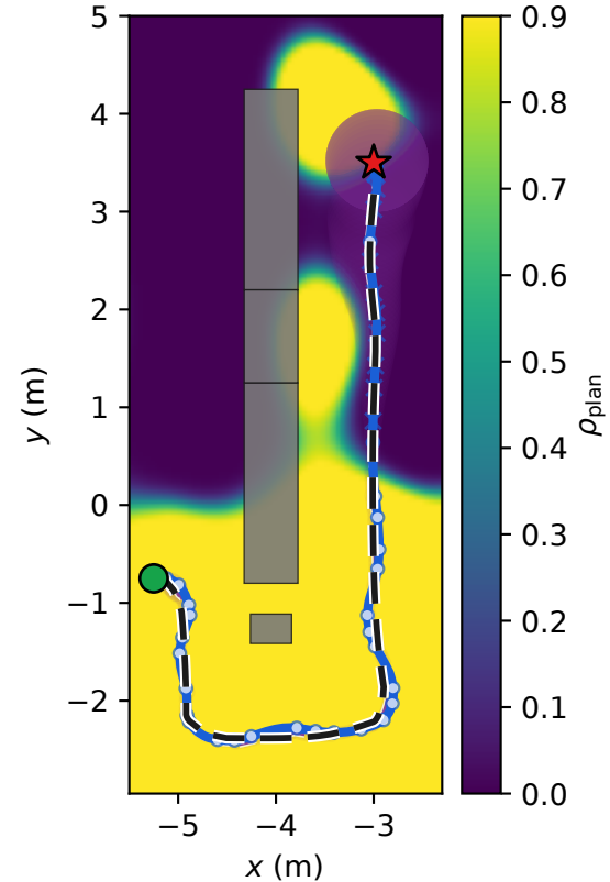
(b) Current C2: visible detour succeeds
