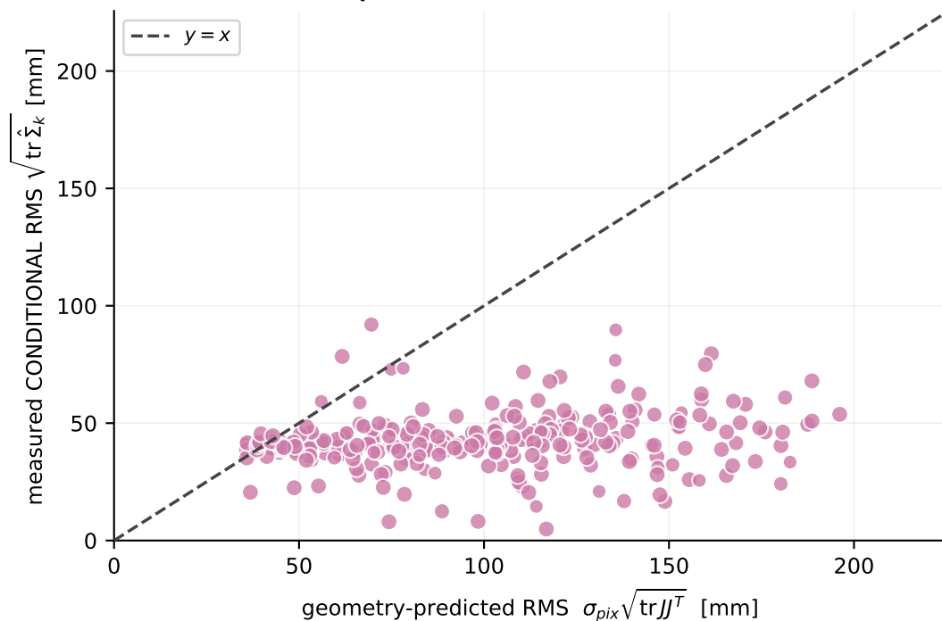
(b) does geometry predict the local SPREAD? N = 2431 detections · M = 306 cells (0.5 m, \geq 5 each) conditional: R^2 vs identity = -32.95 · cell Spearman = +0.25 · median obs/pred = 0.46 median per-cell BIAS removed first = 44 mm
