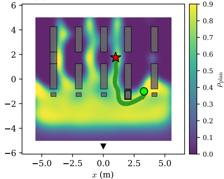
(b) Learned covariance — seed 0
