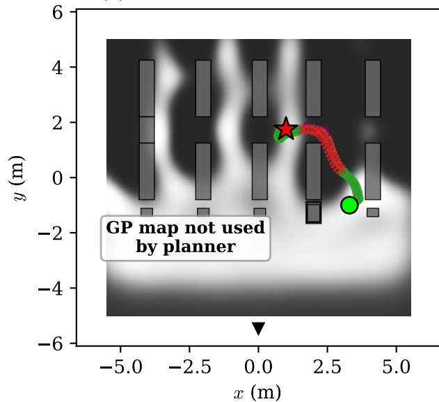
(a) Constant covariance — seed 0
