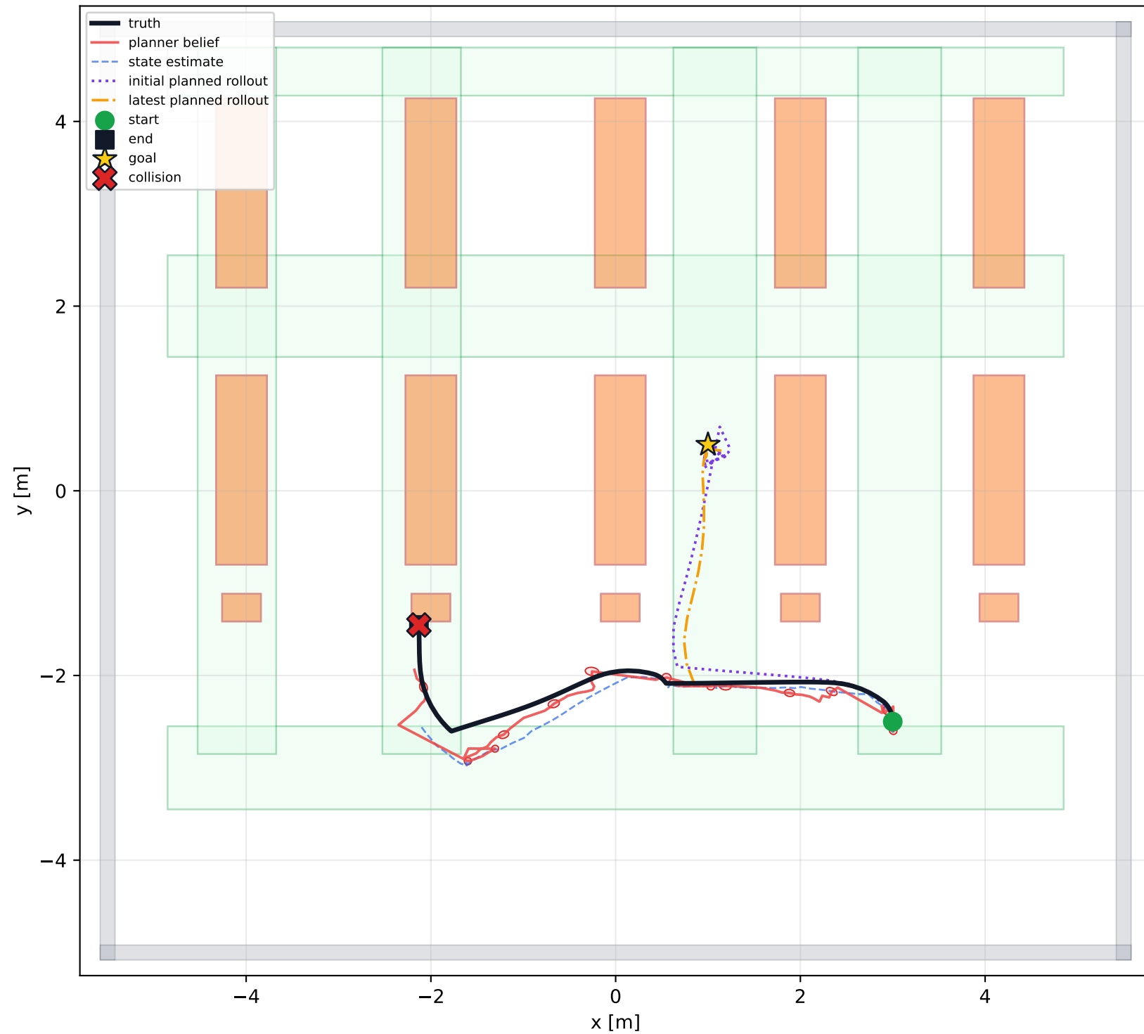
(a) Map: trajectory, belief, plans, collision geometry
