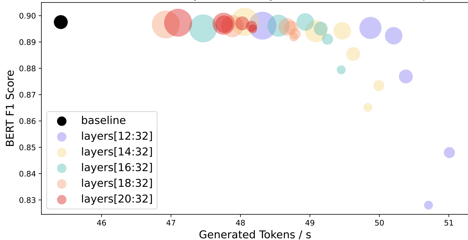
VQA BERT F1 Score by Masked Layers and Number of Samples
